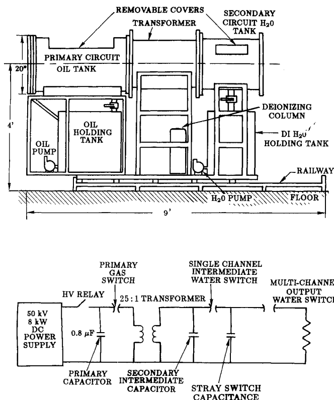
Figure 1. Compact 1 MV pulser.
