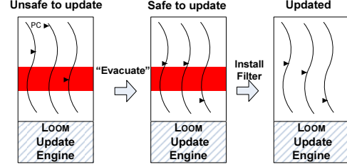
Figure 9: Evacuation . Curved lines represent application threads, solid triangles (in black) represents the threads’ program counters (PC), and solid stripes (in red) represents an unsafe code region.
