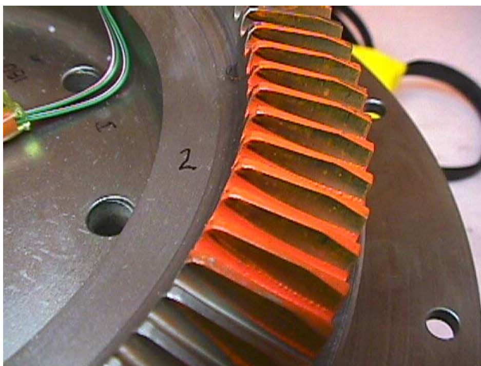
Figure 24. Idler 4 Contact Patterns with Upper and Lower Face Gears Full Load Contact Pattern Inspection
