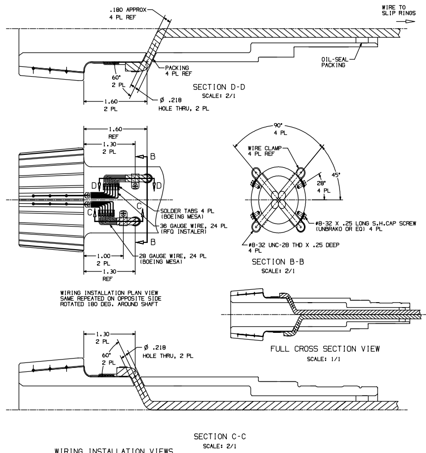
INPUT PINION STRAIN GAGE AND WIRE INSTALLATION
