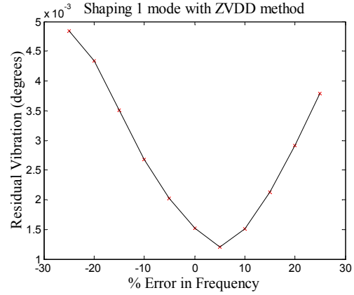
Figure 13. Effect of percentage frequency error on the maximum residual vibration, applying PI control (using rate feedback) with torque feedforward and input shaping 1 mode with ZVDD method
