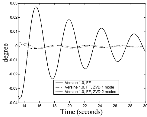
Figure 11. Residual vibration from using versine profiles with input shaping of 0, 1, or 2 modes (using ZVD method). (PID control with rate feedback, and torque feedforward applied in all three cases)
