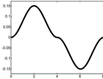
Figure 4. Versine Torque profiles without input shaping
