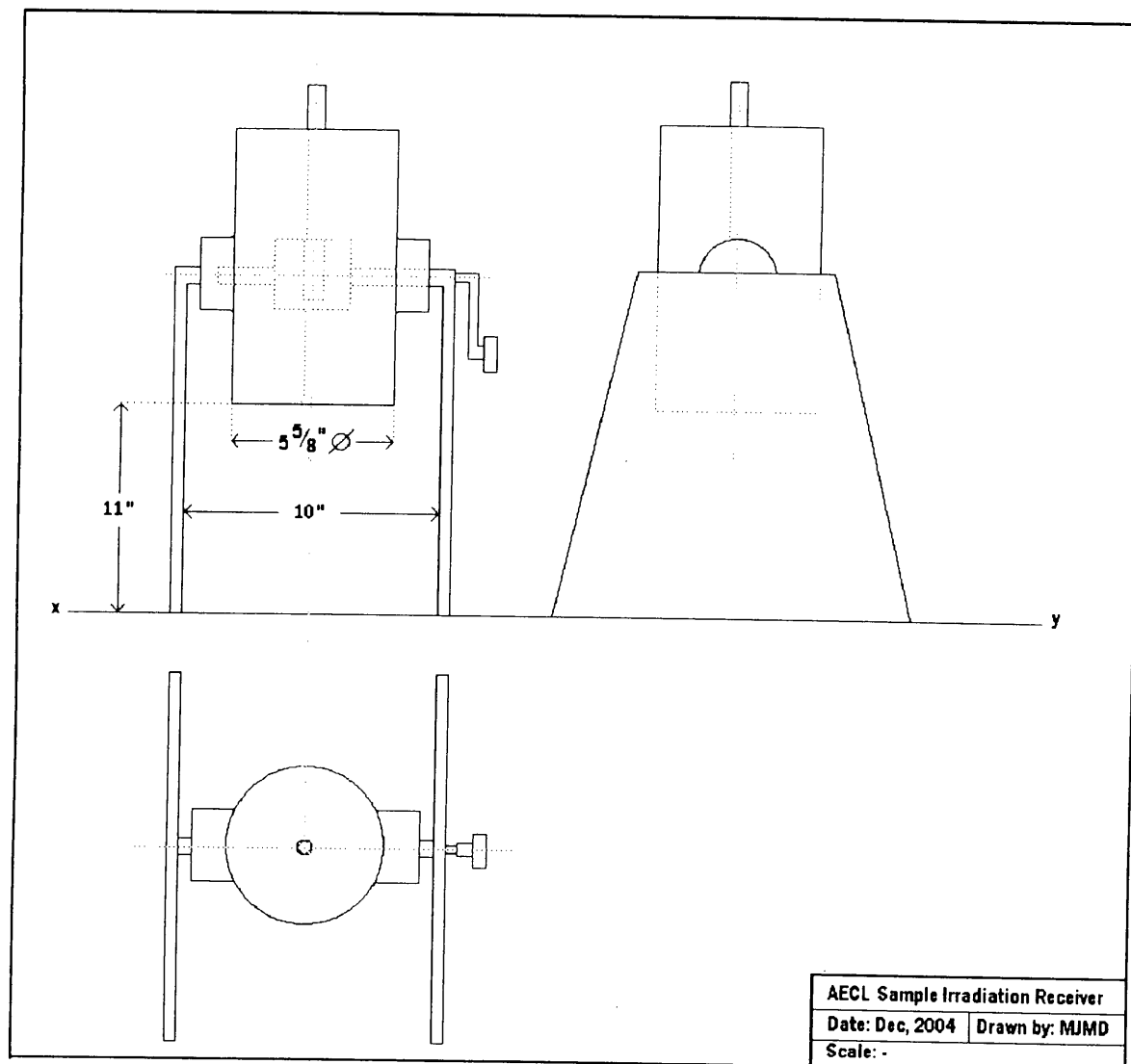
Figure 1. AECL Sample Irradiation Receiver.
