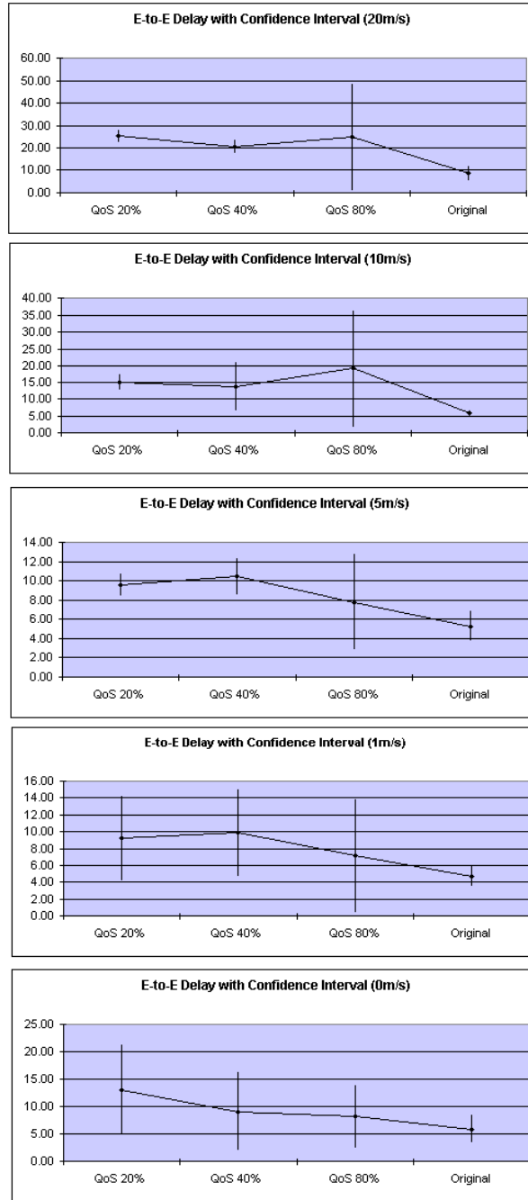
Figure 20: End-To-End Delay Comparison with Confidence Intervals
