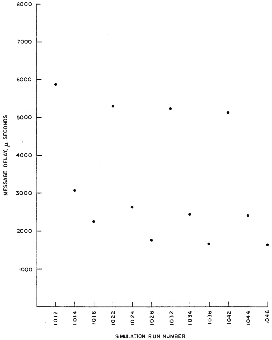
Figure D-2. Global Bus Network Simulation Overall Mean Message Delay, \mu Seconds Using RN1 Random Number Seed 10 Run Series
