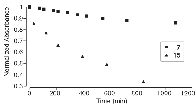
Figure 4. Comparison of the disappearance of monomers 7 and 15 over time (100 mM NH 4 Ac buffer, pH 6.75, 25 °C).
