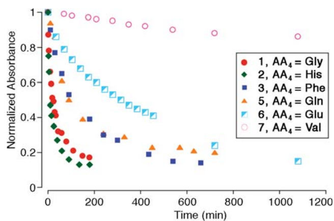
Figure 3. Plot of the disappearance of monomers 1–3 and 5–7 over time (100 mM NH 4 Ac buffer, pH 6.75, 25 °C).
