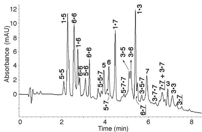
Figure 5. HPLC trace of a mixture of 1 , 3 , and 5–7 after equilibration for 1 h (100 mM NH 4 Ac buffer, pH 6.75, rt). Underlined species indicate linear oligomers.
