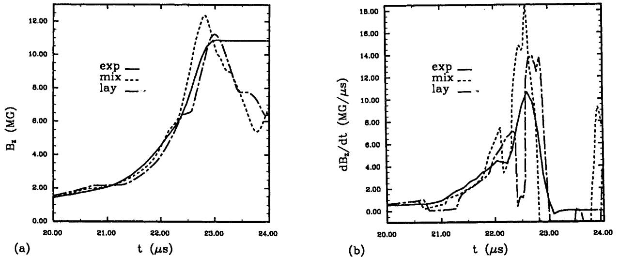
Fig. 5. Calculated field (MG) (a) and field derivative (MG/ \mu s ) (b) for PBX-9501 using the mixed EOS and layered model for cascades compared to experimental data.
