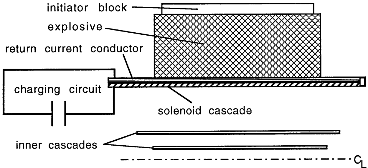
Fig. 1. Schematic cross-section of the Russian three-cascade coaxial MC-1 FCG.
