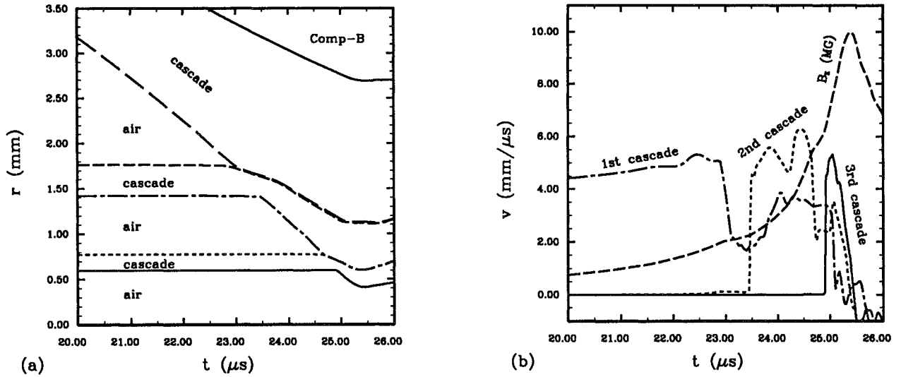
Fig. 2. Cascade radii (a) and velocity (b) for Comp-B simulations using the mixed EOS. Calculated field is overlaid in (b).
