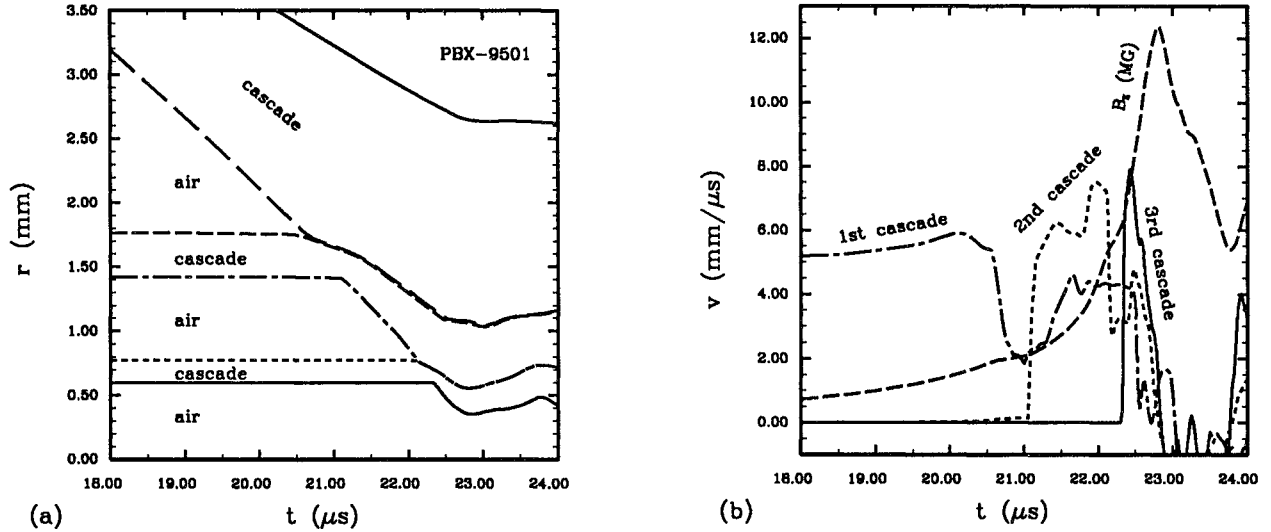
Fig. 3. Cascade radii (a) and velocity (b) for PBX-9501 simulations using the mixed EOS. Calculated field (MG) is overlaid in (b).
