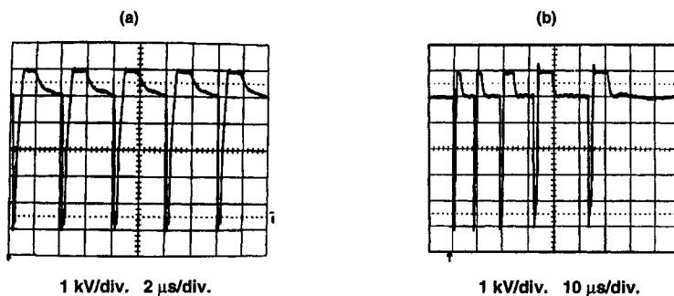
Figure 5. (a) Five-pulse burst of 200-ns pulses at a maximum rate of 250 kHz. (b) Five-pulse burst of variable pulses to show machine agility.
