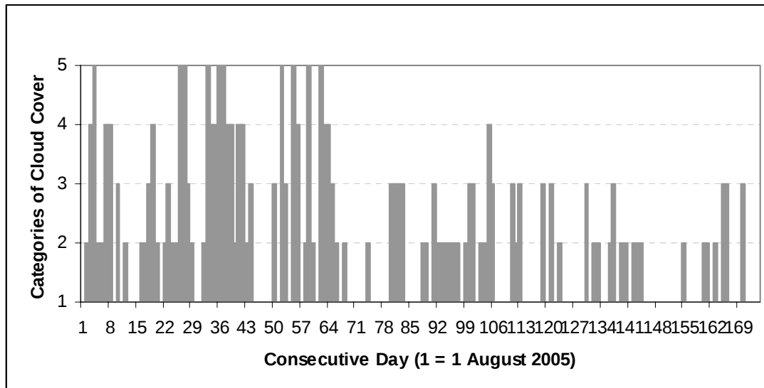
Figure 9. Temporal resolution of MODIS/Terra Aeronet_Halifax images described in Figure 8. Category 1 = 100 % cloud cover or no image; 2 = > 50 % cloud cover; 3 = 25 to 50 %; 4 = < 25 % and 5 = virtually clear image. The 174 consecutive day period runs from 1 August 2005 to 21 January 2006.
