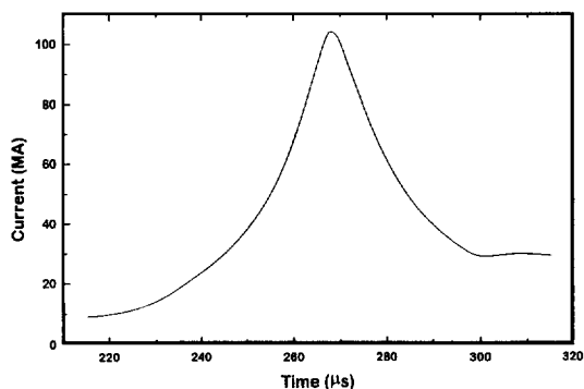
Figure 2. Typical experimental current pulse, starting with onset of DEMG operation; I_{\text{max}} = 104 \text{ MA} .
