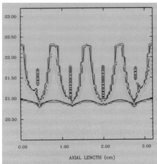
Figure 4. Density contours for typical 2-D MHD calculation with initial perturbations on outer edge; A = 240 \mu\text{s} , \lambda = 8 \text{ mm} .
