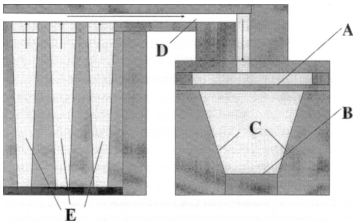
Figure 1. Experimental configuration for HEL-1: (A) Aluminum Amg-6 alloy liner, (B) central measuring unit (CMU), (C) steel electrodes/glidesplanes, (D) power flow channel, (E) disk electromagnetic generator (DEMG) modules.
