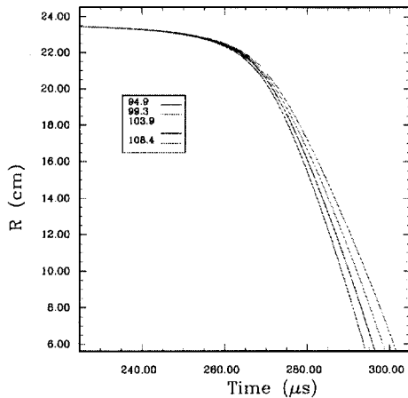
Figure 3. Radius of inner edge of liner profile versus time for I_{\text{max}} = 94.9, 99.4, 103.8, 108.4 MA, (1-D MHD).
