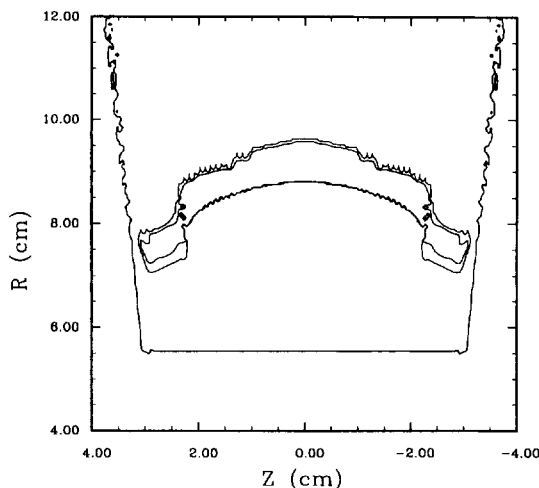
Figure 5. Density contours for a liner/glide plane 2-D MHD calculation near impact with CMU; I_{\max} = 99.4
