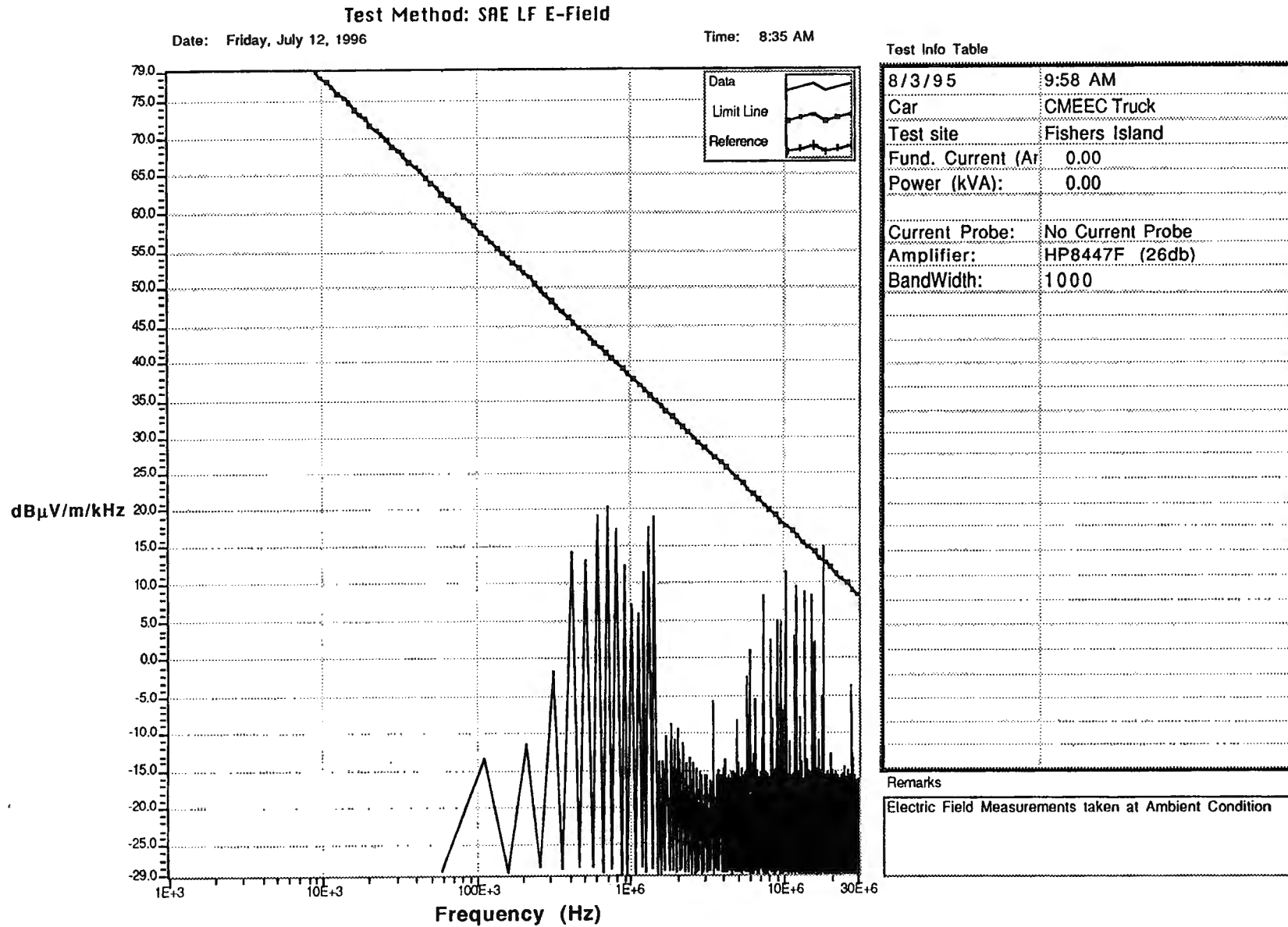
Figure 4. CMEEC Vehicle in Open Field, E Field (0.014-30 MHz) Taken at Ambient Condition
