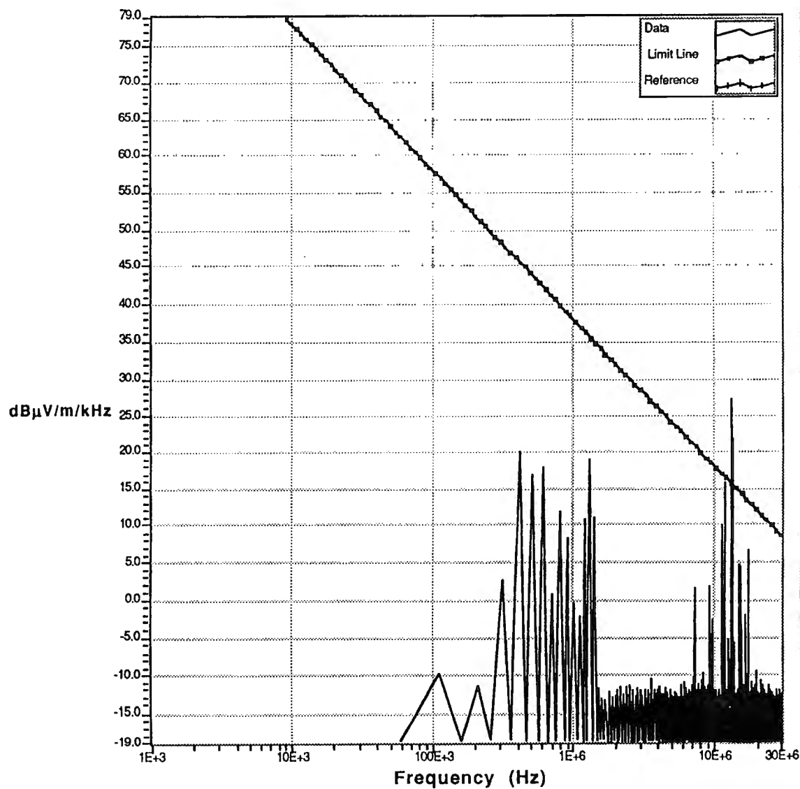
Figure A-27. Solectria Force Vehicle in Open Field, E Field (0.009-30 MHz) Taken at Ambient Condition
