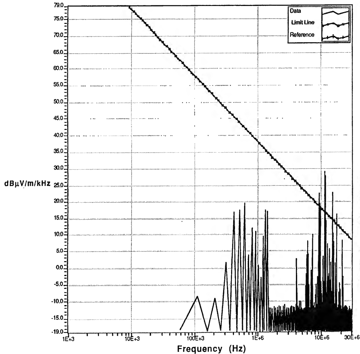
Figure A-28. Solectria Force Vehicle in Open Field, E Field (0.009-30 MHz) Taken 10 m from the Front Side
