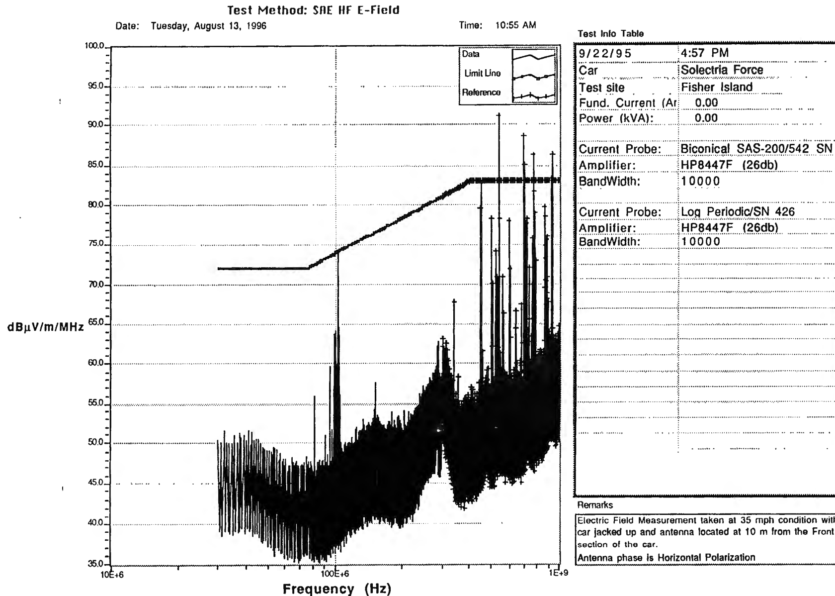
Figure A-30. Solectria Force Vehicle in Open Field, E Field (30-1000 MHz) Taken 10 m from the Front Side
