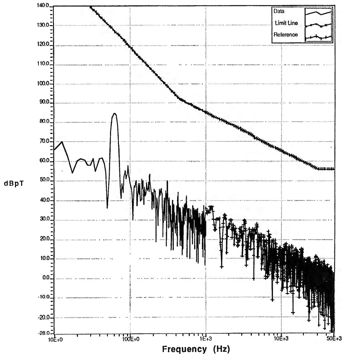
Figure A-19. Dodge Dakota Vehicle in Open Field, B Field Measurements Taken at Ambient Condition
