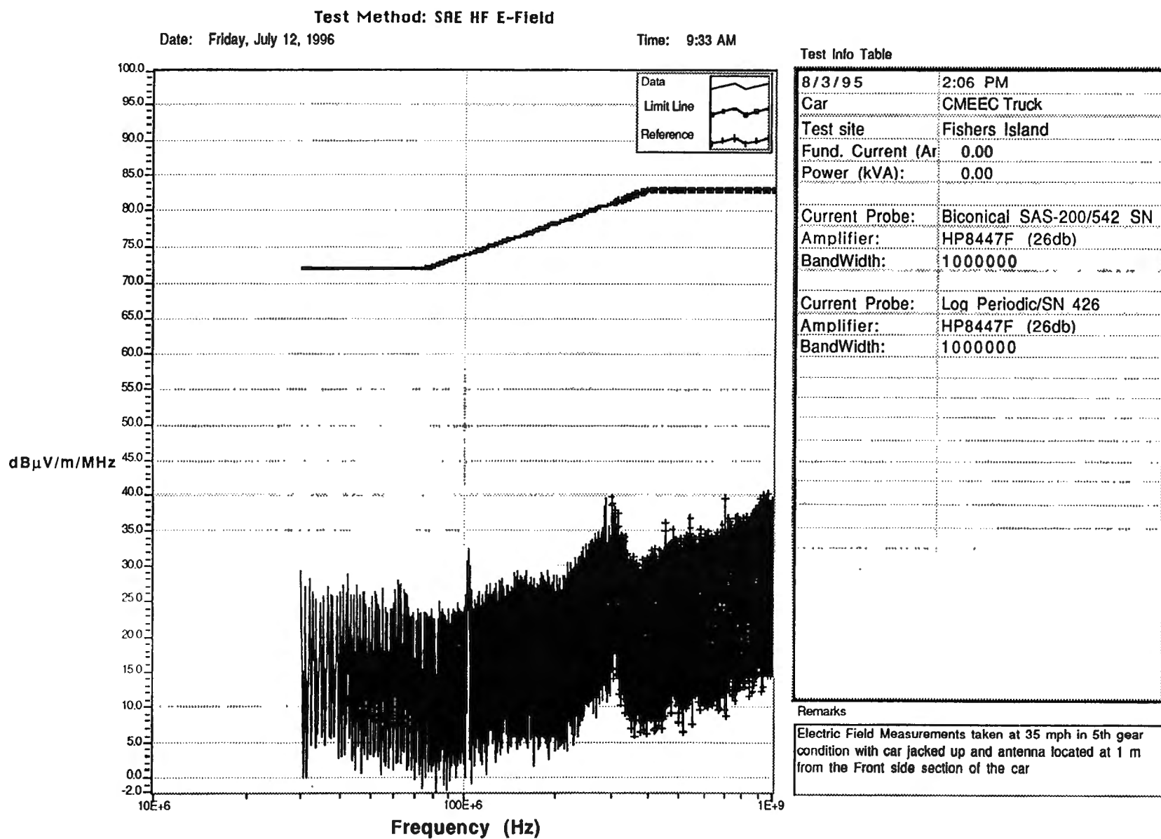
Figure 10. CMEEC Vehicle in Open Field, E Field (30-1000 MHz) Taken 1 m from the Front Side
