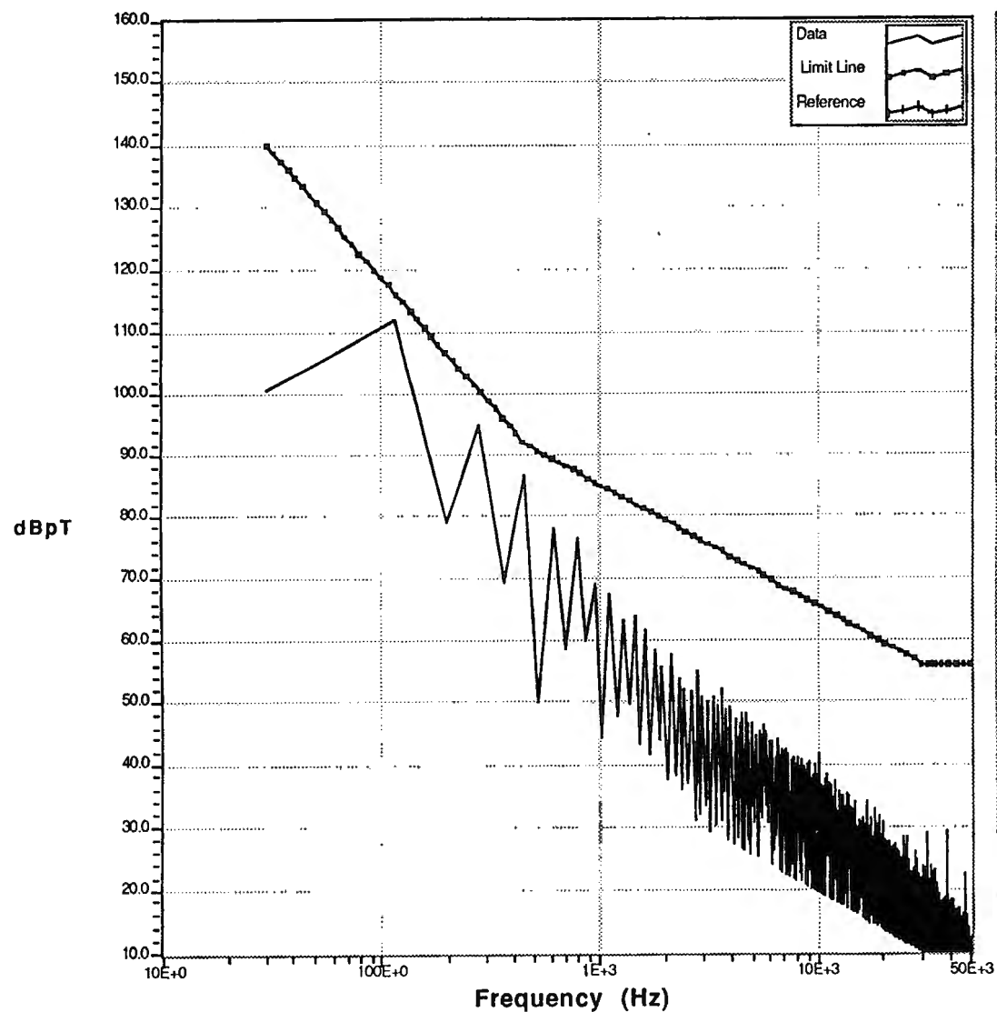
Figure 8. CMEEC Vehicle in Open Field, B Field Measurements Taken 1 m from the Driver's Side
