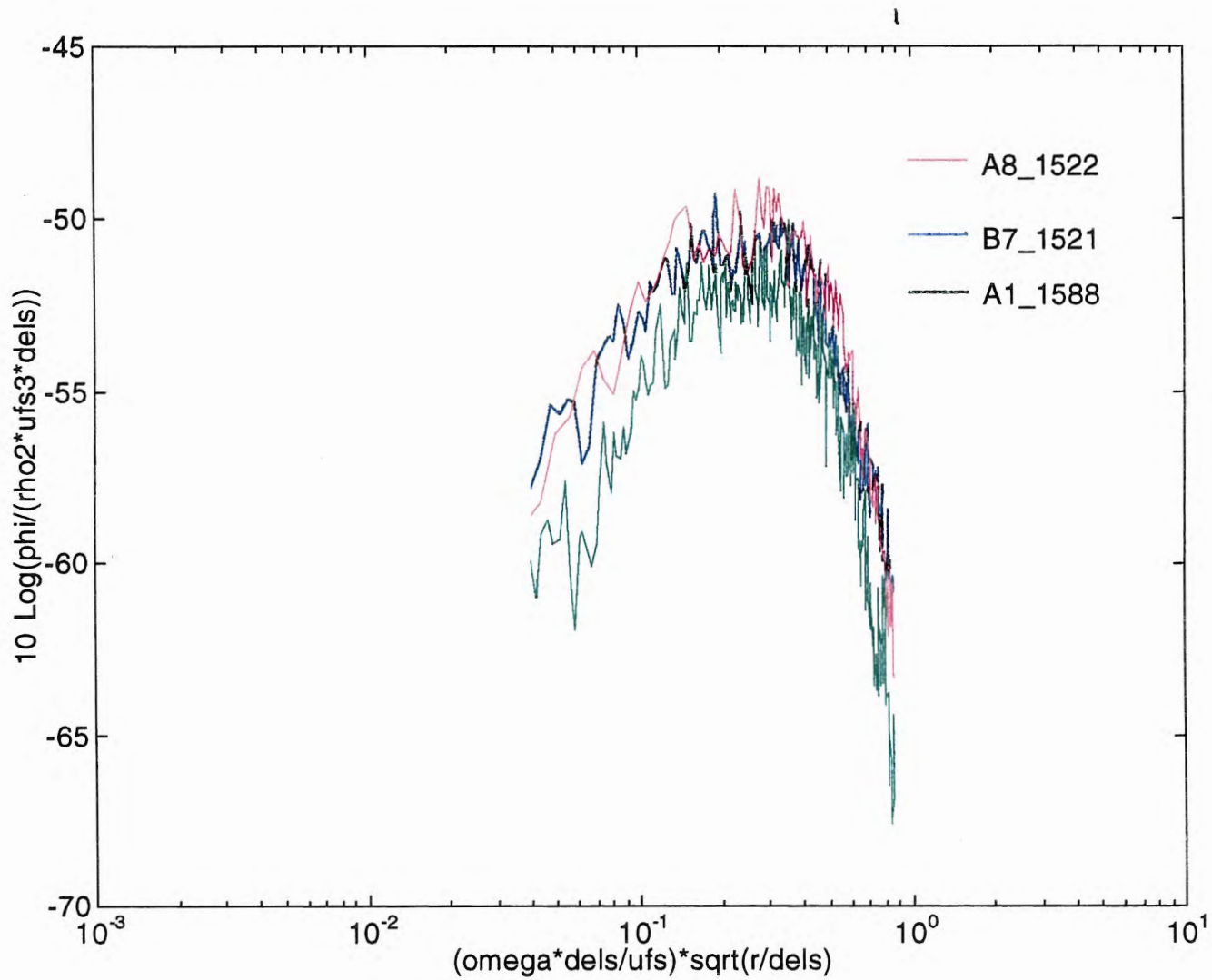
Figure 6: Corcos Corrected Spectra with (r/\delta^*)^{1/2} Frequency Modification (Case 1)
