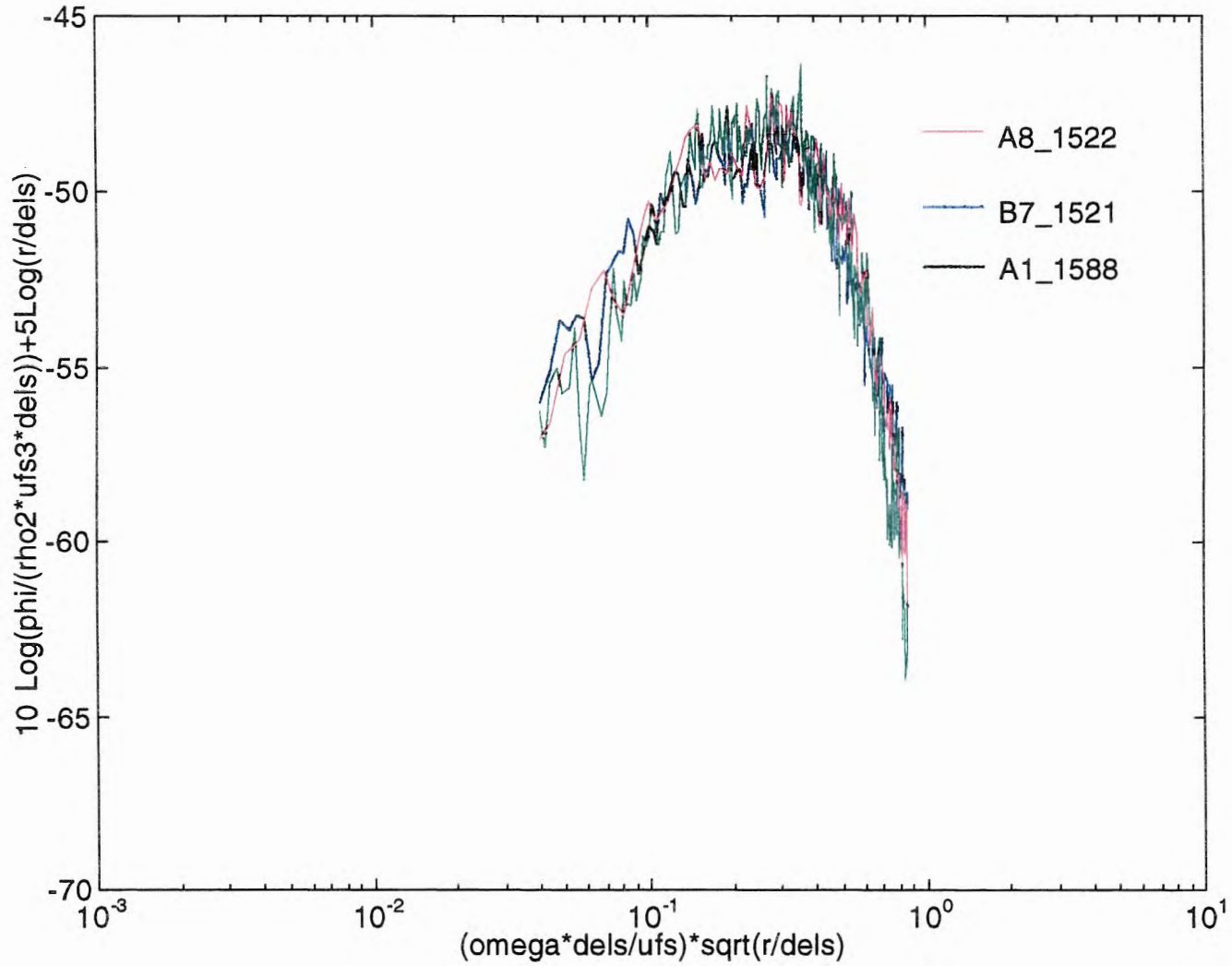
Figure 7: Corcos Corrected Spectra with (r/\delta^*)^{1/2} Frequency and Amplitude Modifications (Case 1)
