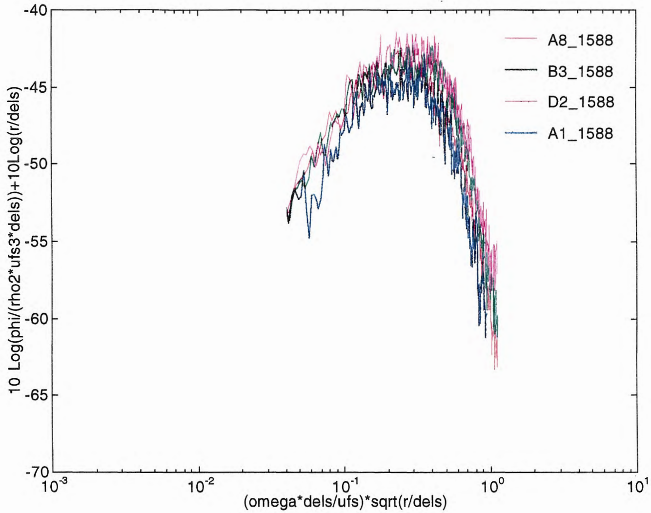
Figure 12: Corcos Corrected Spectra with (r/\delta^*)^{1/2} Frequency and r/\delta^* Amplitude Modifications (Case 2)
