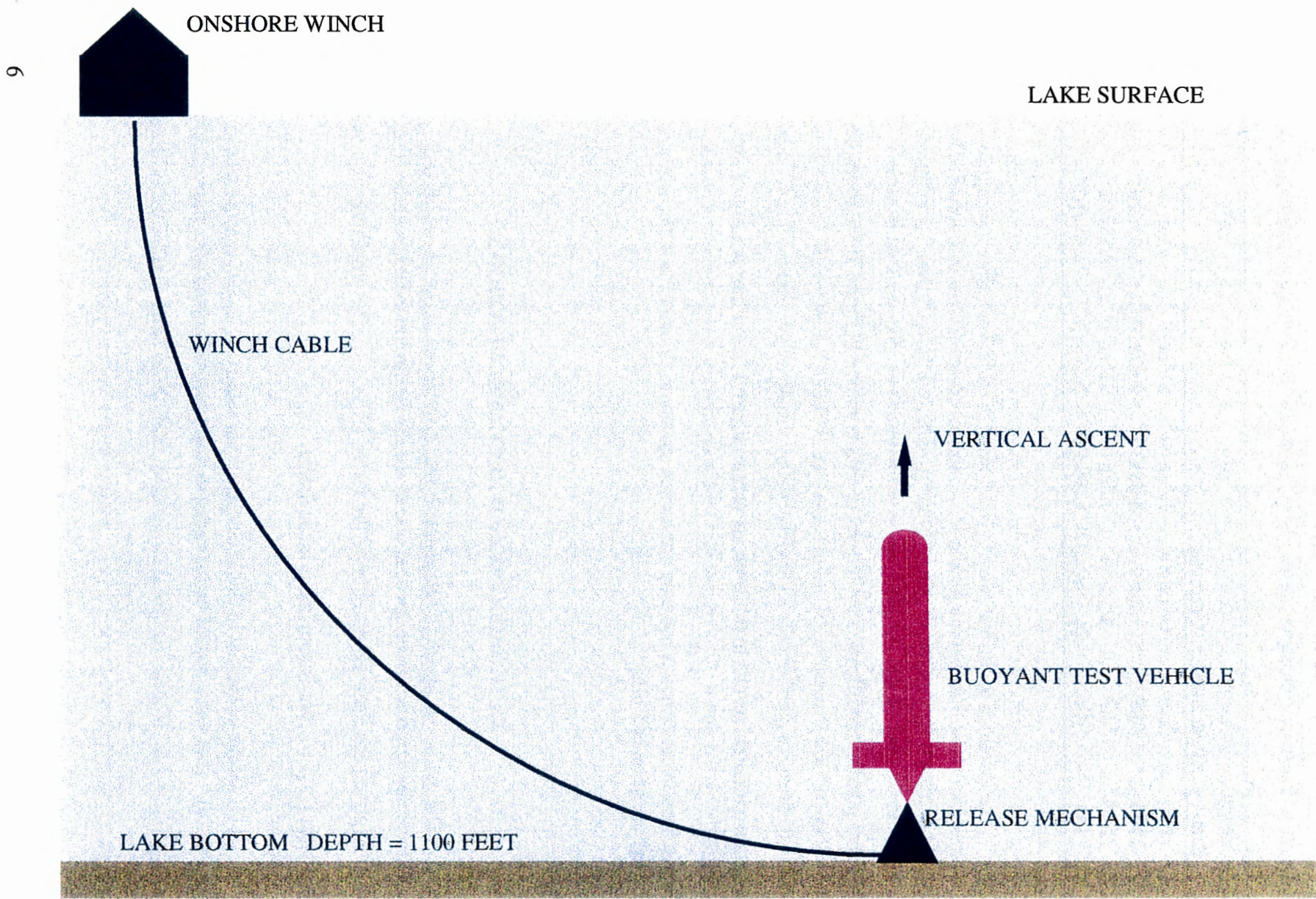
Figure 1: Experiment Setup
