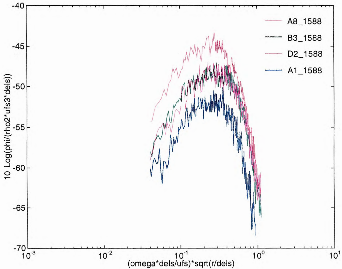
Figure 10: Corcos Corrected Spectra with (r/\delta^*)^{1/2} Frequency Modification (Case 2)
