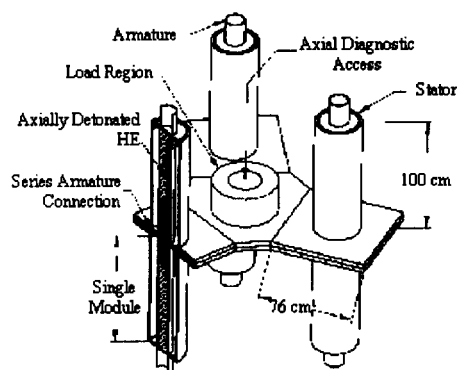
Fig. 1. Ranchero system concept. This system has two series generators in each of three parallel branches. As shown, the system requires ~180 kg explosive and needs a helical booster generator with an additional 50 kg explosive for very high current operation. The module currently under development is 140-cm long, which would increase the total explosive to 250 kg + 50 kg.
