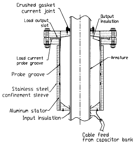
Fig. 5. Test configuration ("B") with end output load. Faraday probes in the load current probe grooves survive past peak current. The armature is 43 cm in length.
