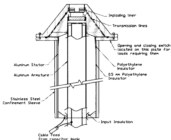
Fig. 2. Single 1.4 m Ranchero Module with Atlas-like load attached. The explosive is detonated 56 places along the 1.4 m axis.
