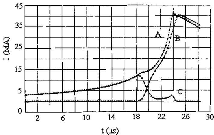
Fig. 7. Circuit model calculation of a Ranchero module with an opening switch and load isolation switch to protect the liner load from the early current foot. Curve A is the module current, curve B is the load current, and curve C is the opening switch current. The opening switch in the calculation is a resistance profile that is plausible from experience, and requires no extension of technology to create.
