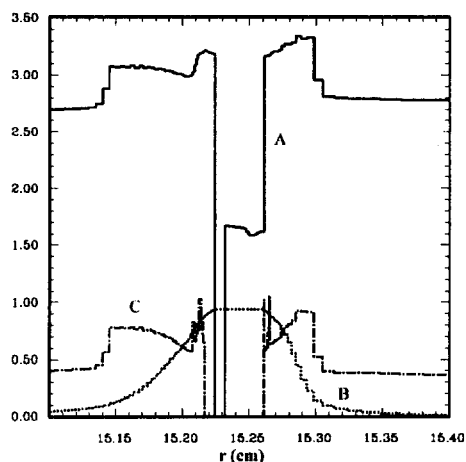
Fig. 3. RAVEN calculations of density in \text{g/cm}^3 (A), magnetic field in units of \text{T} \times 10^{-1} (B), and yield strength in \text{J/cm}^3 (C) for the Ranchero armature and stator at a time near collision.
