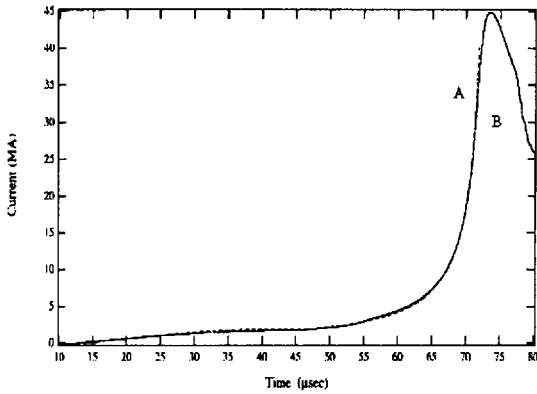
Fig. 6. Current waveforms from two tests. For consistency, we show the two Faraday rotation probes even though the fiber in Test A failed because of shockwave in its location. A dB/dt probe fitted to the early Test A curve yields a peak current of 48 MA on that test. Consistency between the two curves is very good until the effects of the tapered stator become important. The taper gives rise to \sim 1 \mu\text{s} longer operation with reduced dI/dt during the last 1 \mu\text{s} .
