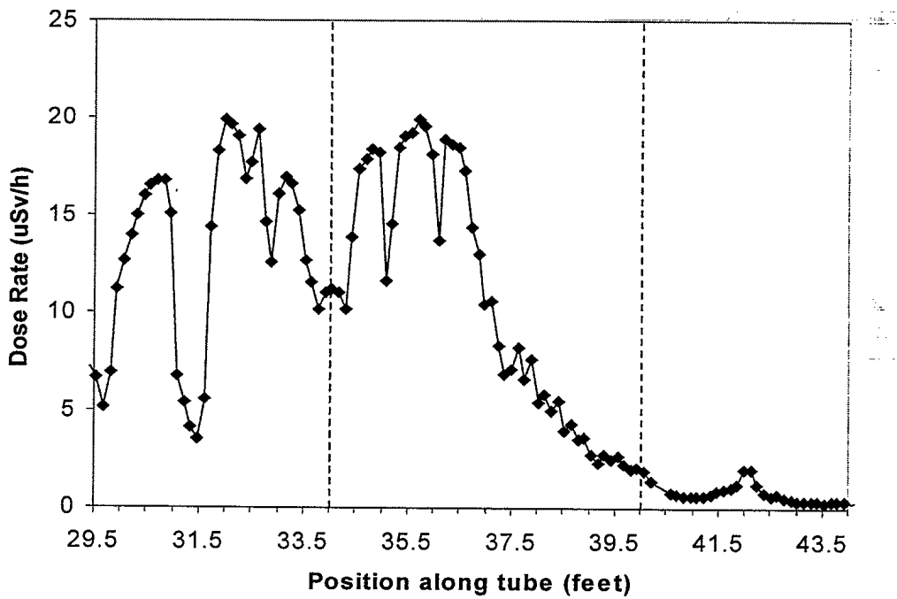
Figure 11: Dose rate versus source position, with the tube six feet from the front of the vehicle.
