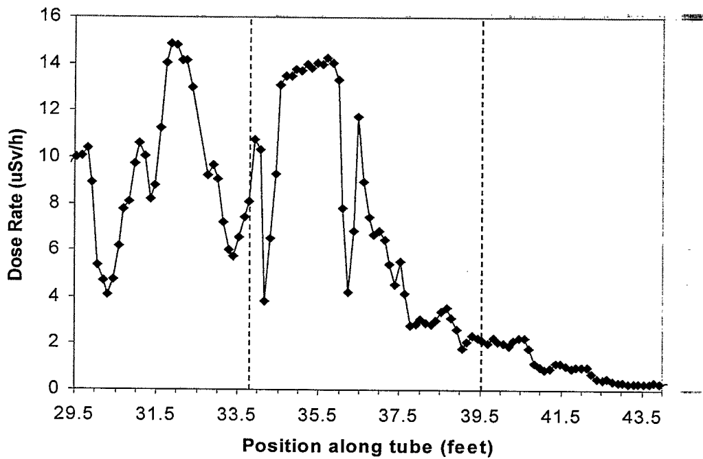
Figure 12: Dose rate versus source position with the tube seven feet from the front of the vehicle.
