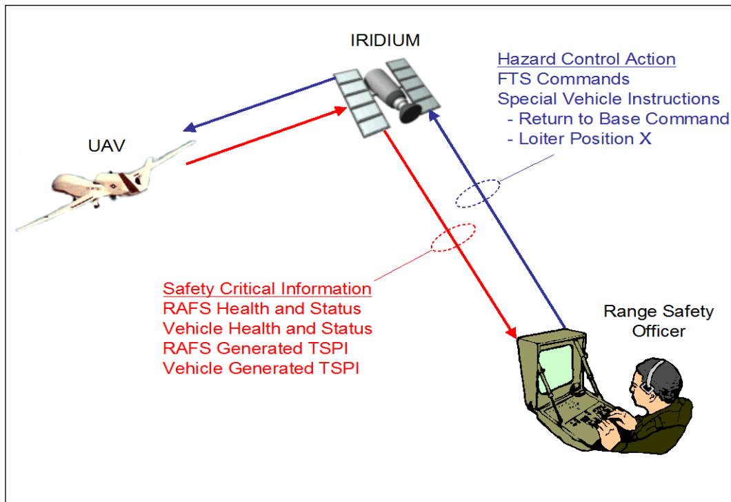
Figure 1-1. RAFS Concept.
