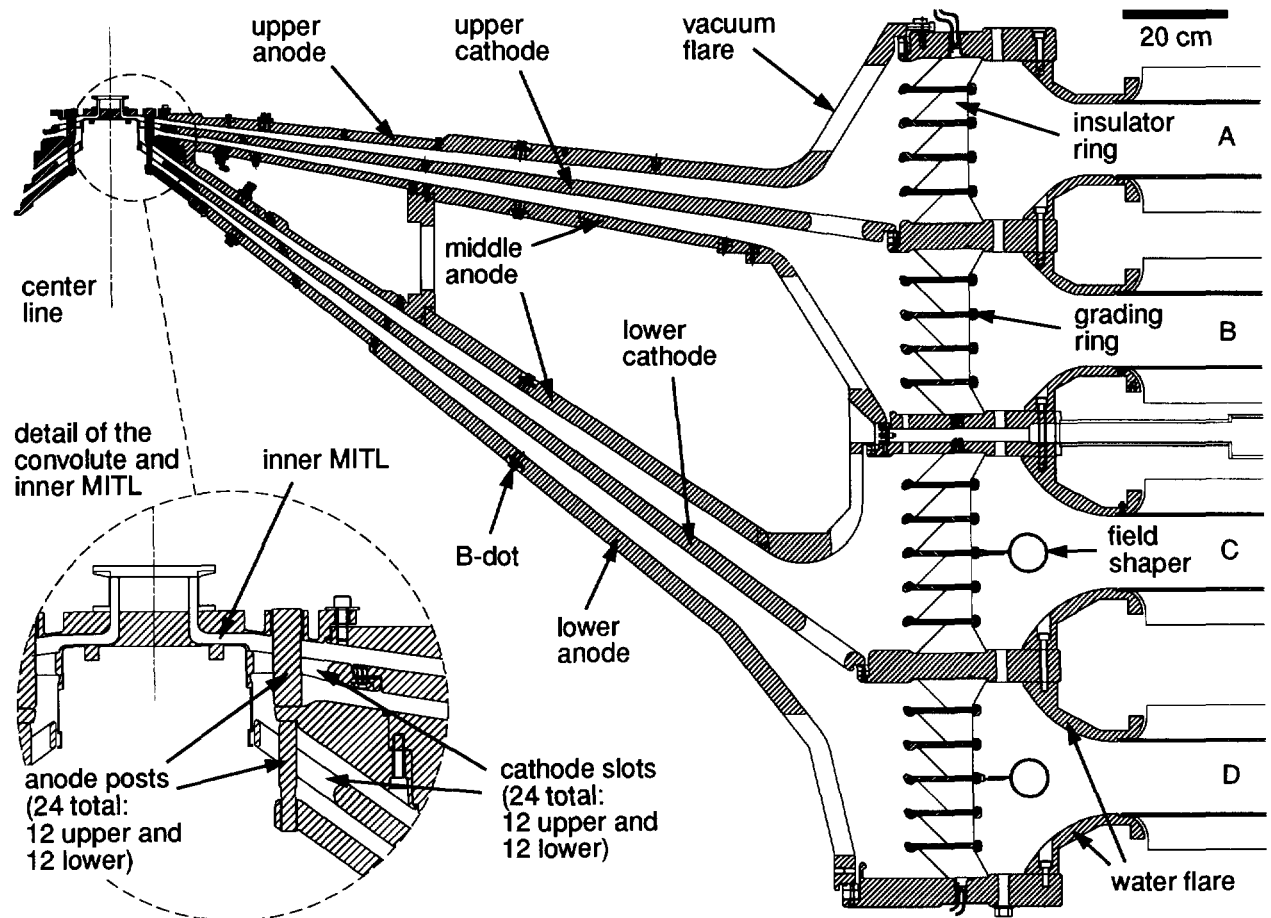
Figure 2. The Z vacuum section.
