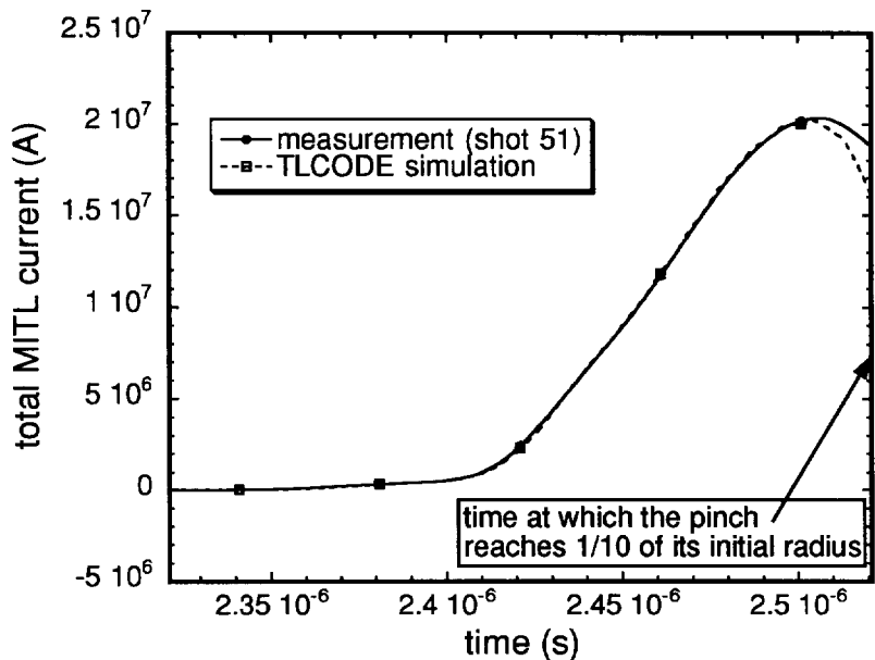
Figure 3. Measured and simulated MITL currents for Z-shot 51.
