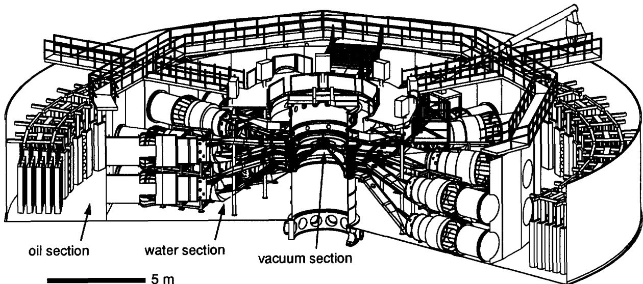
Figure 1. The Z accelerator.
