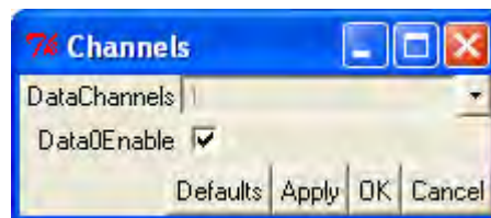
Figure 6-3. Channels Window
