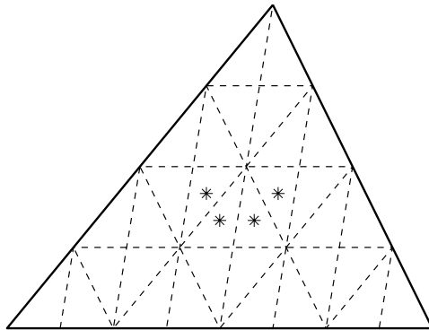
Figure 7.1: Application of the NEW SUBDIVISION RULE to a triangle
