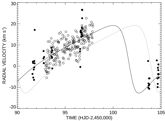
FIG. 1.—Radial velocities derived from the line wings of the UV cfs (open circles) and H \alpha and He I \lambda 6678 (average) (filled circles). The dotted line shows the prediction from T95, while the solid line shows the same curve translated in time to match better the observations.
