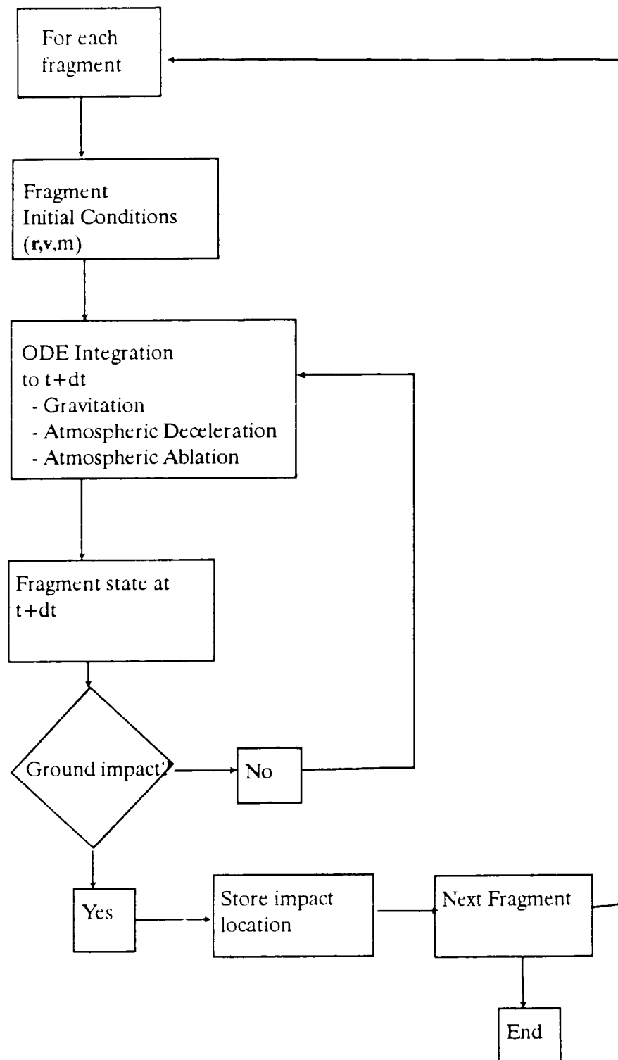
Figure 4: Fragment Re-Entry Module - Conceptual Flow
