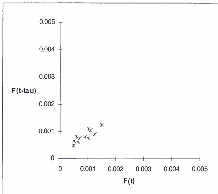
Figure 23. Poincaré map for the normalized WWII casualties. 85 The two-dimensional cross section is of a three-dimensional phase space constructed by a time delay of one and eight days.
