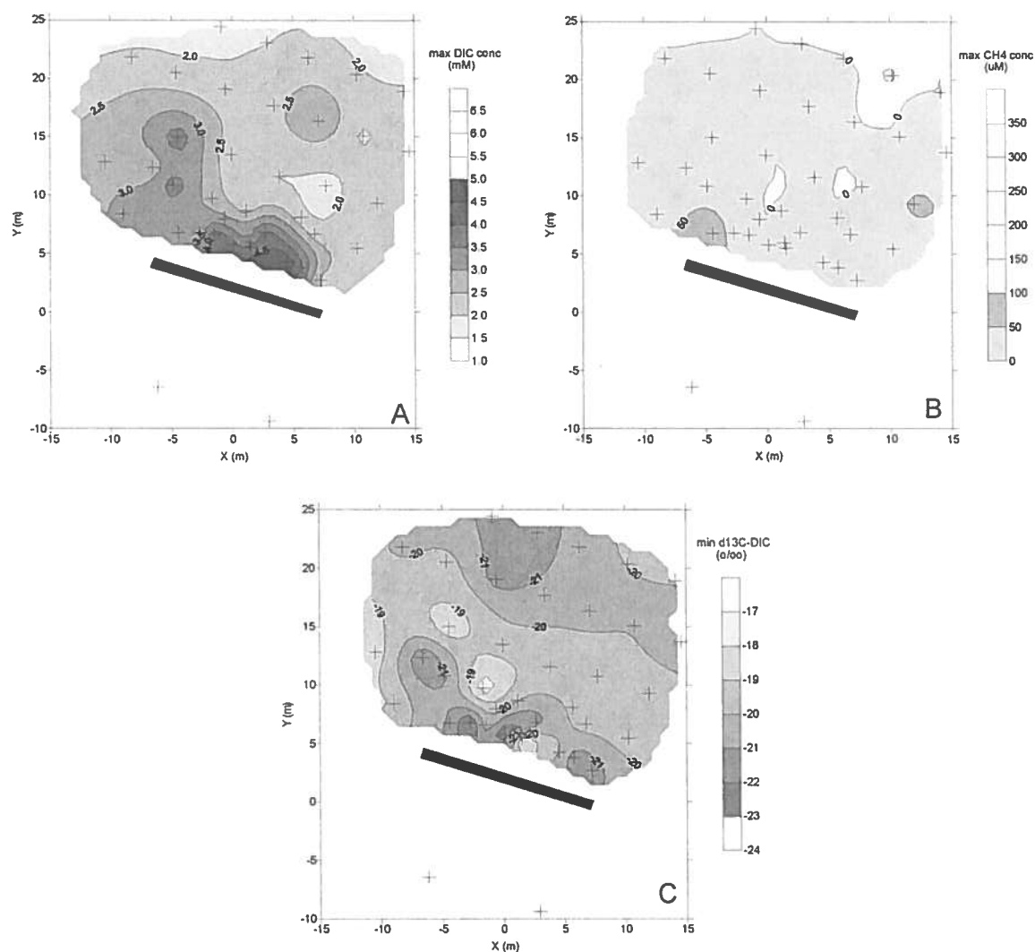
Fig. 5. Contour maps showing DIC (A) and \text{CH}_4 (B) concentrations and DIC \delta^{13}\text{C} (C) in groundwater in September 1996, 278 days after the November 1995 hydrocarbon contamination. Maximum concentrations and minimum isotopic signatures were used to represent maximum extent of degradation. The black rectangular box located in the upgradient section of field represents the trench containing the hydrocarbons.
