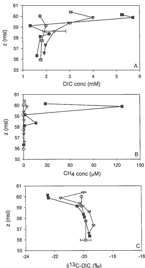
Fig. 7. Temporal vertical profiles of DIC and CH 4 concentrations and δ 13 C at a multi-level sampler located 4.2 m down-gradient of the hydrocarbon source (M013). The vertical axis is in terms of msl (meters above sea level) with land surface located at 65 msl. Groundwater contamination was initiated in November 1995. Open circles represent samples collected in September 1995, 100 days prior to contamination; open triangles, September 1996, 278 days after contamination; and filled squares, March 1998, 831 days after contamination.
