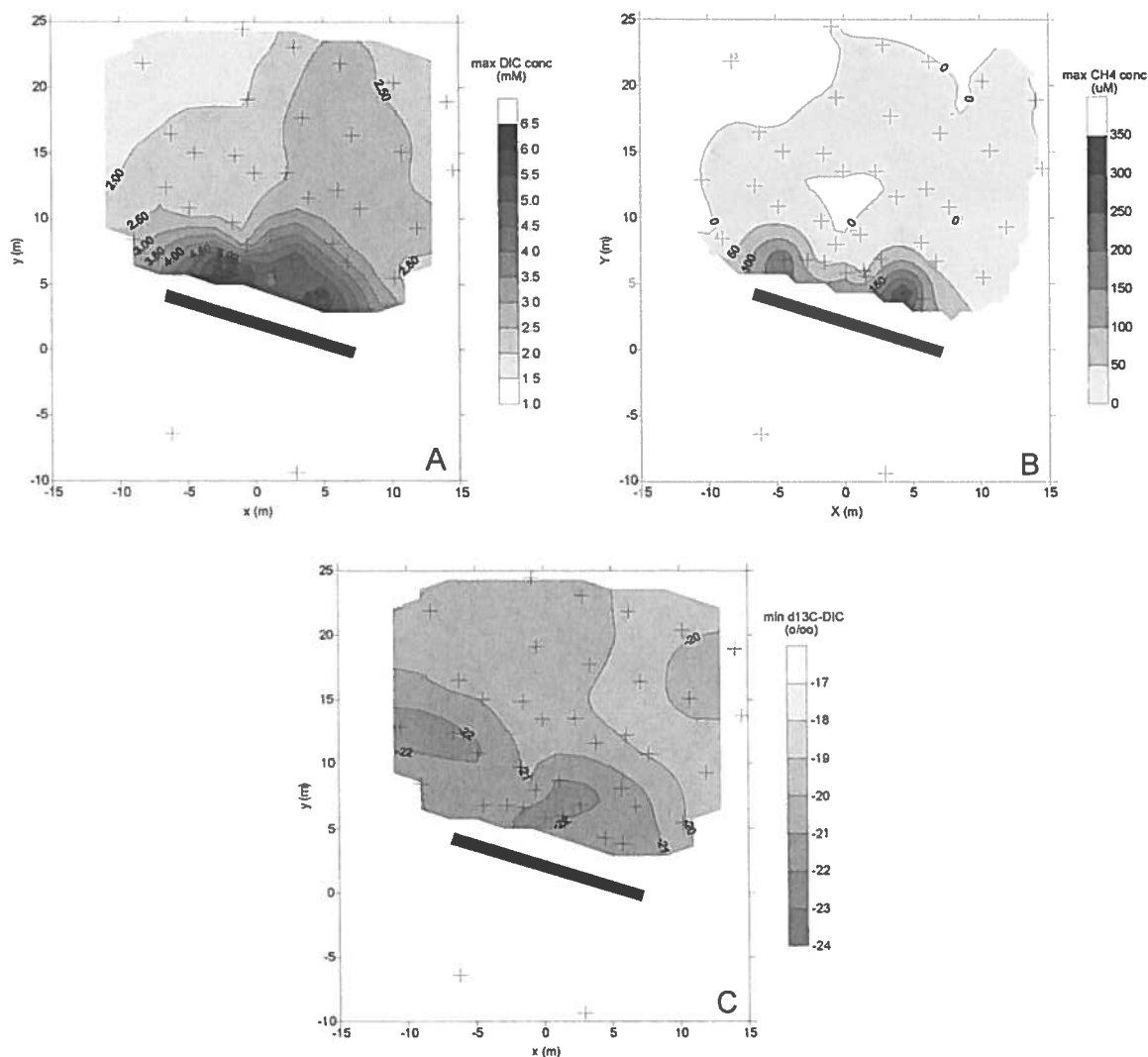
Fig. 6. Contour maps showing DIC (A) and CH 4 (B) concentrations and DIC \delta^{13}\text{C} (C) in groundwater in March 1998, 831 days after contamination. Maximum concentrations and minimum isotopic signatures were used to represent maximum extent of degradation. The black rectangular box located in the upgradient section represents the trench containing the hydrocarbons.
