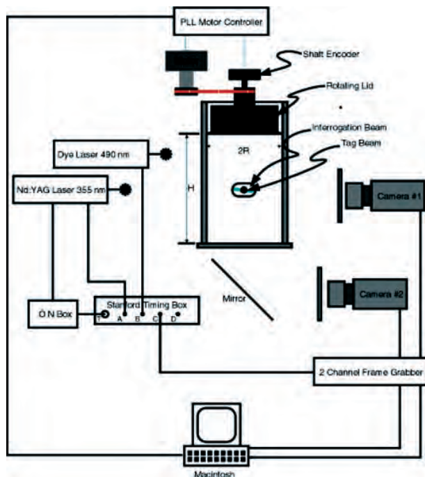
Figure 3. A simplified schematic diagram of the lid driven cylinder flow apparatus.
