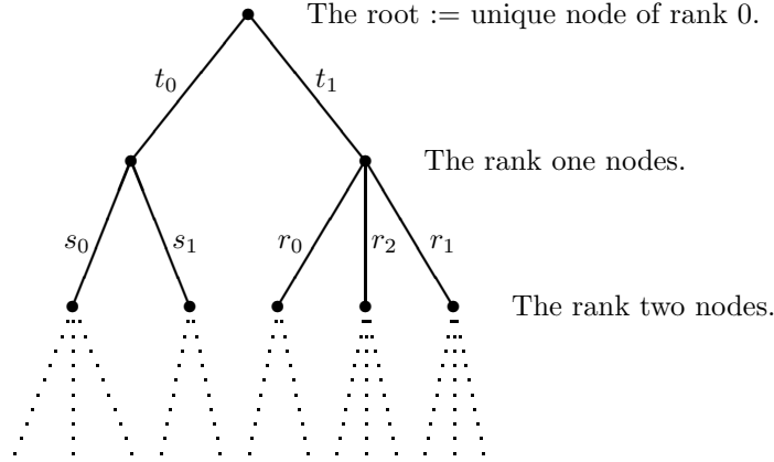
FIGURE 1. An S ranked tree showing the labeling of the edges out of the root by t = (t_0, t_1) \in S and the edges out of the rank one nodes by s = (s_0, s_1) \in S and r = (r_0, r_1, r_2) \in S . In our definition each node will have at least two edges leaving it and the sum of the weights t_0, \dots, t_m of the weights of all edges leaving a node is unity (as (t_0, \dots, t_m) \in \Delta_m ). Finally, in the definition of tree used here, all branches are of infinite length.
