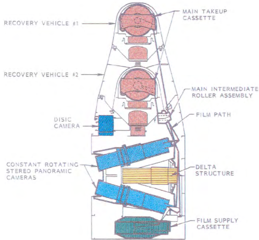
Major Components of the J-3 System
