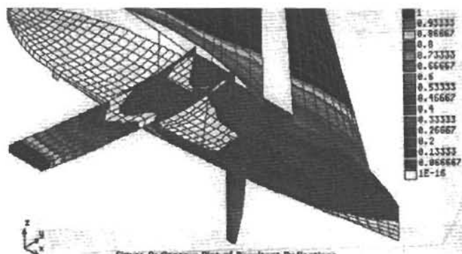
Fig. 9 Contour plot of resultant deflections
