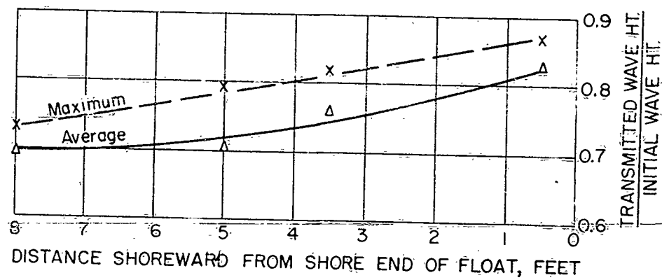
VARIATION OF H_t SHOREWARD FROM FLOAT (from TABLE II)
