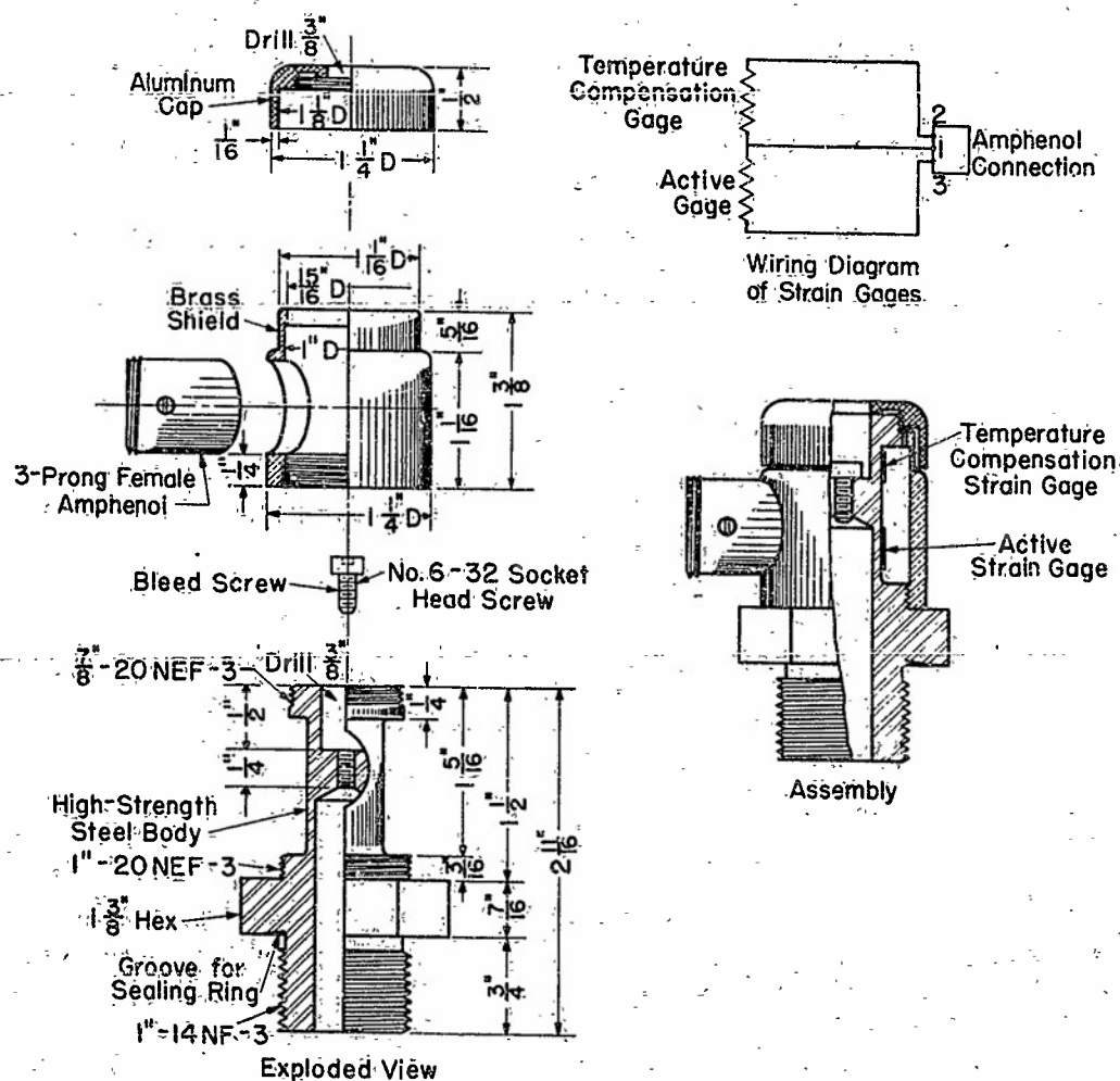
Figure 1 - Schematic Diagram of TMB Elastic-Tube Pressure Gage
