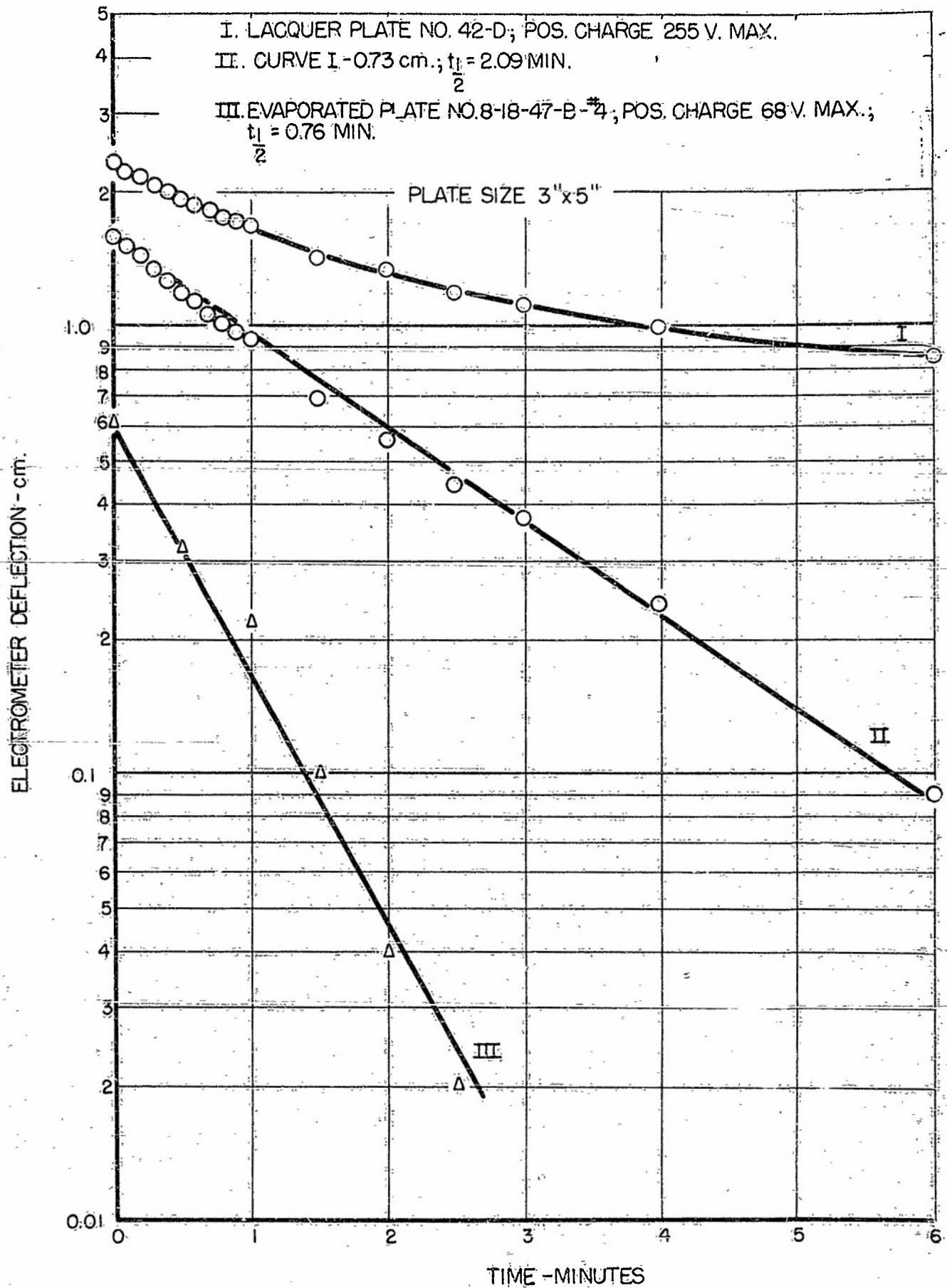
FIGURE 6. DISCHARGE WITH LIGHT SOURCE AS USED FOR STANDARD TESTS ON EVAPORATED PLATES
