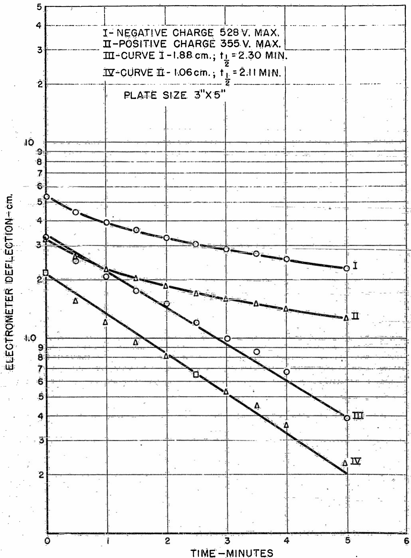
FIGURE 7. DISCHARGE WITH LIGHT SOURCE, AS USED FOR STANDARD TESTS ON EVAPORATED PLATES. LACQUER PLATE NO. 42-G; NO. 3A PAINT WITH LAB. SE.
