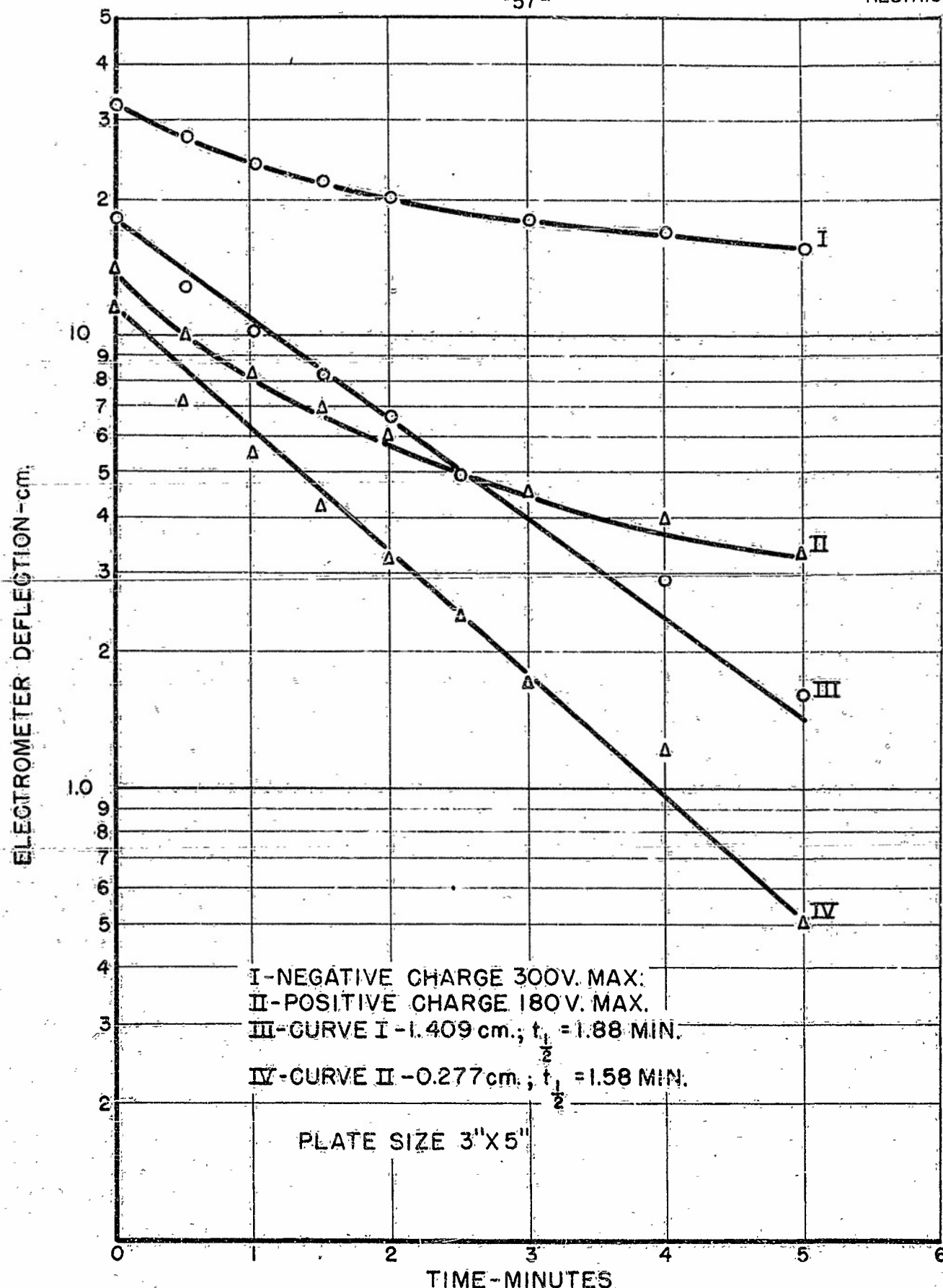
FIGURE 10. DISCHARGE WITH LIGHT SOURCE AS USED FOR STANDARD TESTS ON EVAPORATED PLATES. LACQUER PLATE NO. 3997-4H; NO. 3A PAINT WITH COR POWDERED SE.
