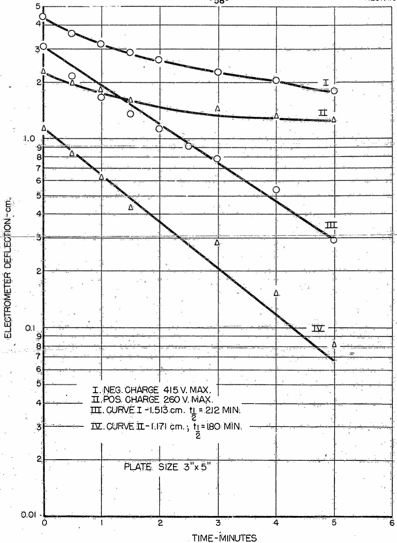
FIGURE 11. DISCHARGE WITH LIGHT SOURCE AS USED FOR STANDARD TESTS ON EVAPORATED PLATES. LACQUER PLATE NO. 3997-41, NO. 3A PAINT WITH CCR, POWDERED SE
