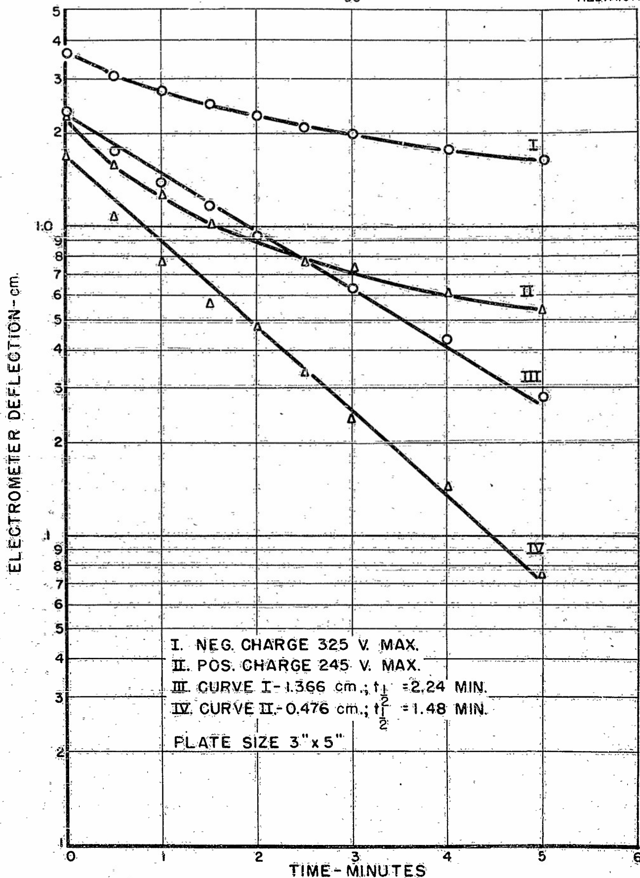
FIGURE 9. DISCHARGE WITH LIGHT SOURCE AS USED FOR STANDARD TESTS ON EVAPORATED PLATES. LACQUER PLATE NO. 3997-46; NO 3A PAINT WITH CCR POWDERED SE.
