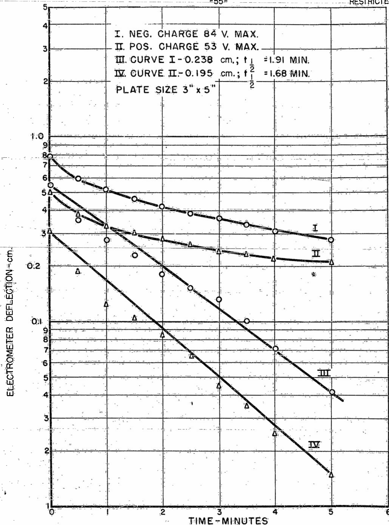
FIGURE 8. DISCHARGE WITH LIGHT SOURCE AS USED FOR STANDARD TESTS ON EVAPORATED PLATES. LACQUER PLATE NO. 3997-3A; NO. 3A PAINT WITH CGR POWDERED SE AND 120% EXTRA REZYL 869
