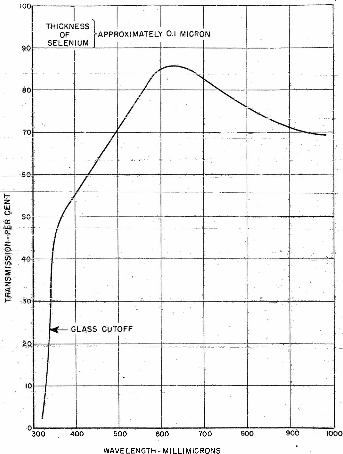
FIGURE 99. TRANSMISSION OF SELENIUM FILM ON GLASS
