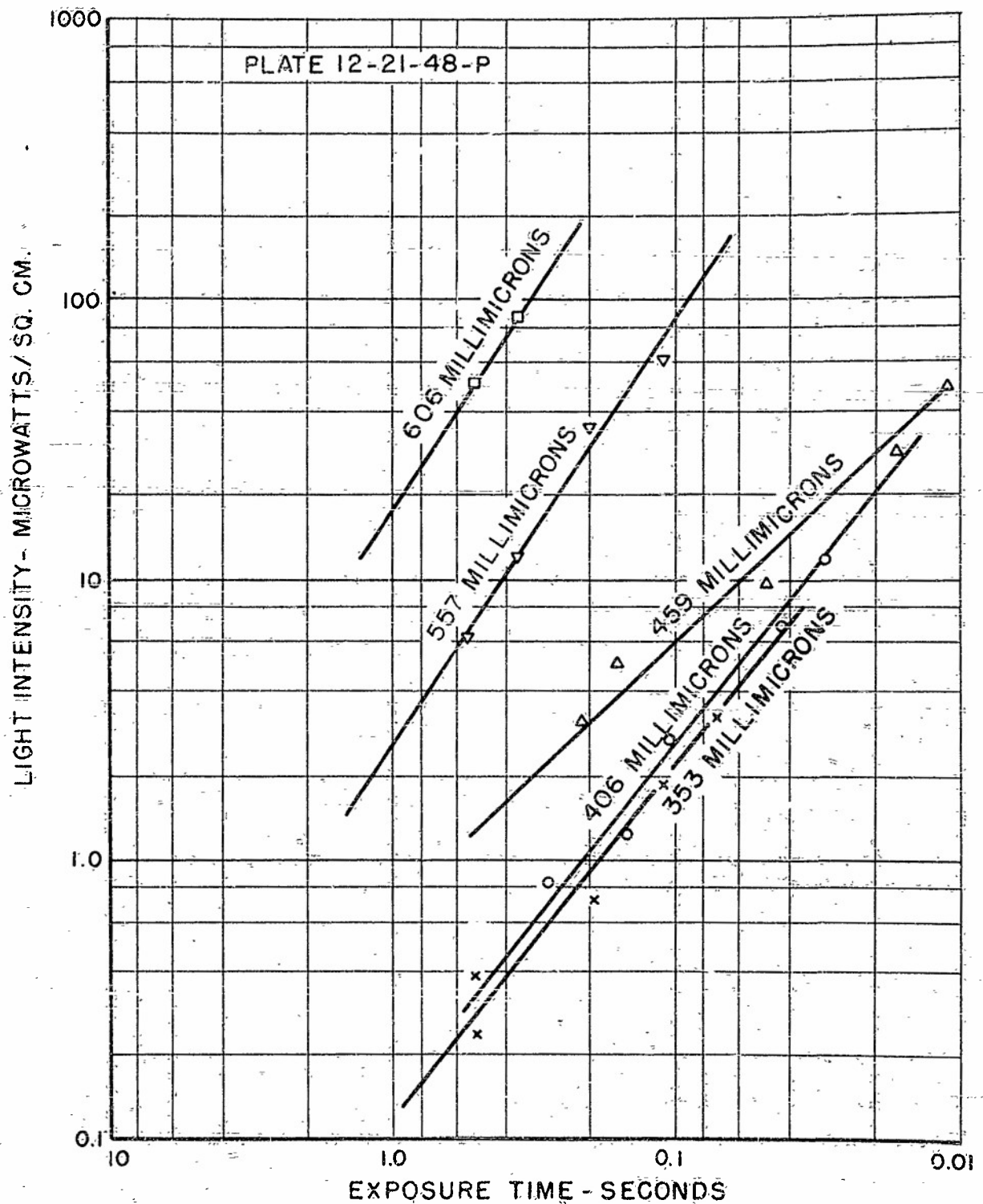
FIGURE 96. RELATIONSHIP BETWEEN LIGHT INTENSITY FALLING ON A SELENIUM-COATED ELECTROPHOTOGRAPHIC PLATE AND EXPOSURE TIME, FOR VARIOUS WAVELENGTHS, NECESSARY TO PRODUCE A NET VOLTAGE DROP OF 100 VOLTS.
