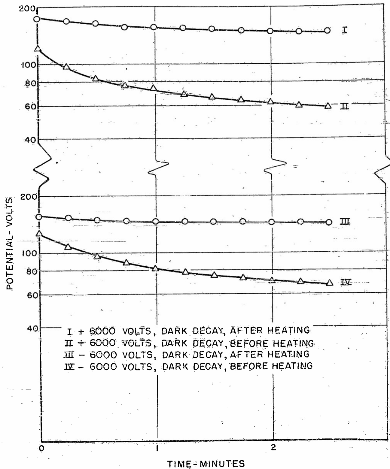
FIGURE 114. EFFECT OF HEATING ON DARK DECAY - PHOSPHOR 2310
