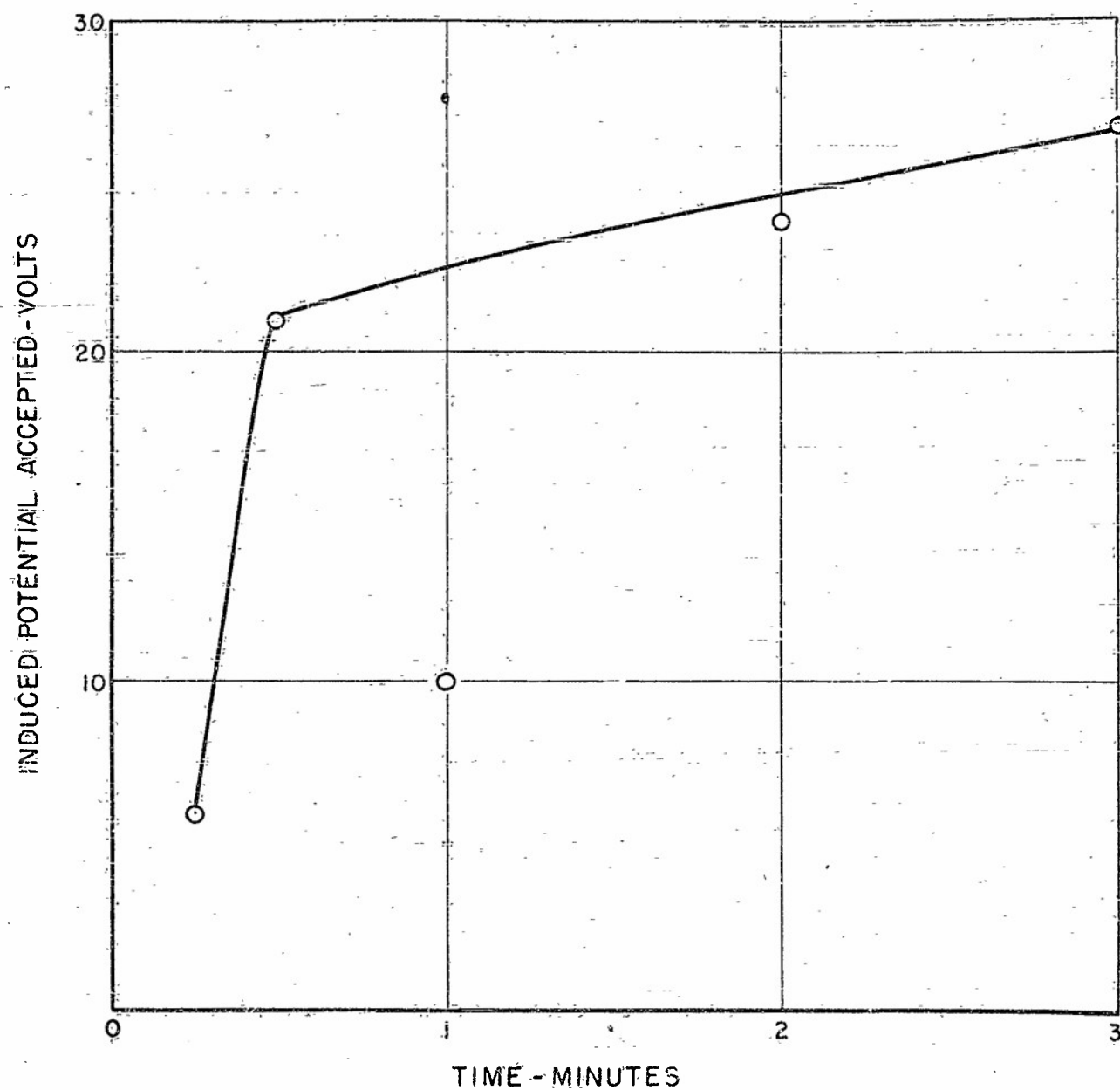
FIGURE 115. DEPENDENCE OF MAGNITUDE OF INDUCED CHARGE ON TIME OF CHARGING - PHOSPHOR 2310
