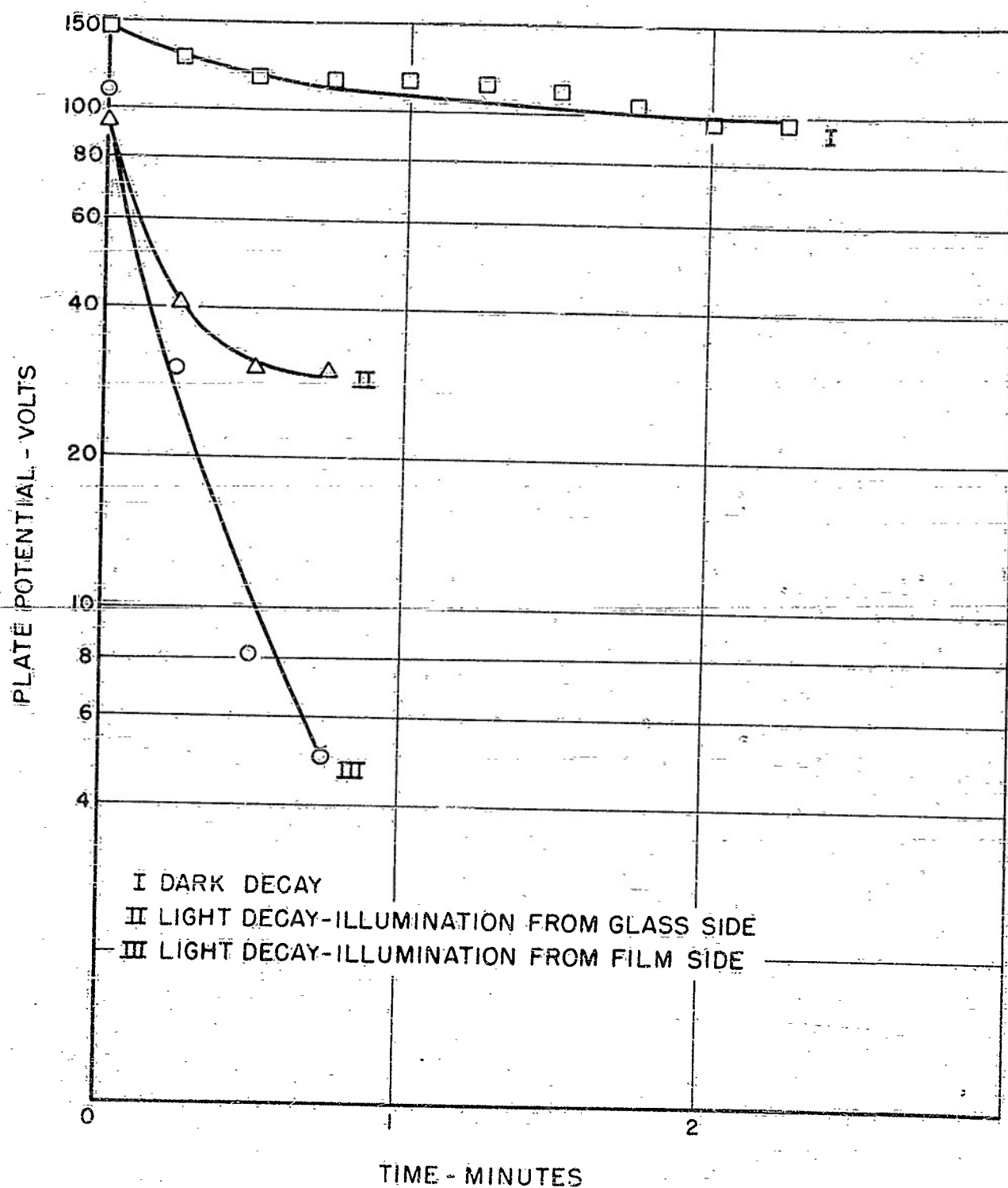
FIGURE 107. POSITIVE- POTENTIAL DECAY CURVES FOR SELENIUM FILM ON ELECTRICALLY CONDUCTIVE GLASS
