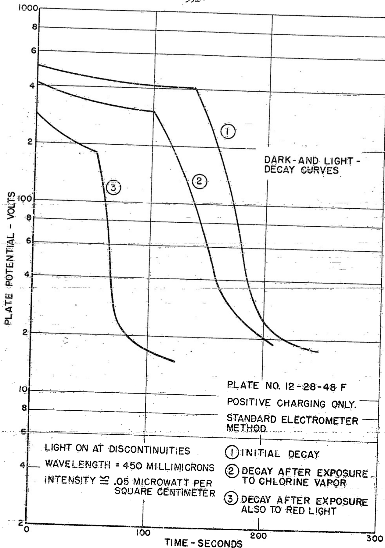
FIGURE 108. POTENTIAL-DECAY CURVES FOR A CHLORINATED SELENIUM PLATE.
