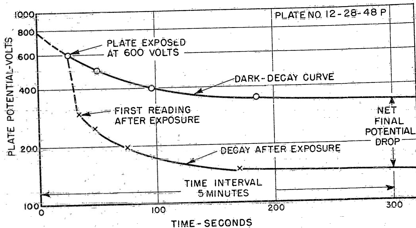
FIGURE 94. DEFINITION OF NET POTENTIAL DROP
