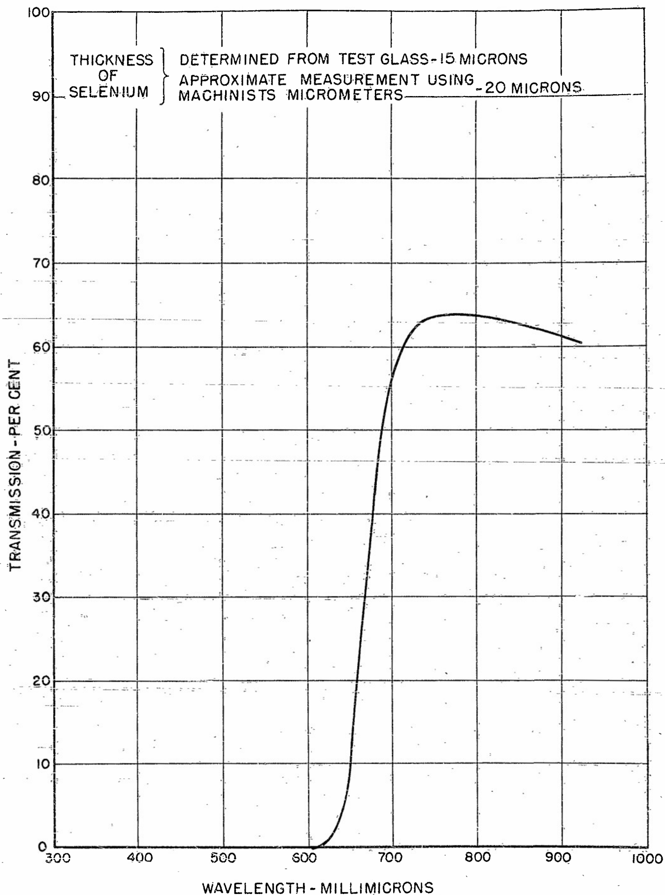
FIGURE 103. TRANSMISSION OF SELENIUM FILM ON GLASS
