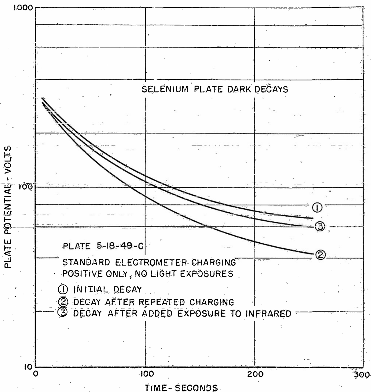
FIGURE 110. EFFECT OF INFRARED IRRADIATION ON A SELENIUM ELECTROPHOTOGRAPHIC PLATE
