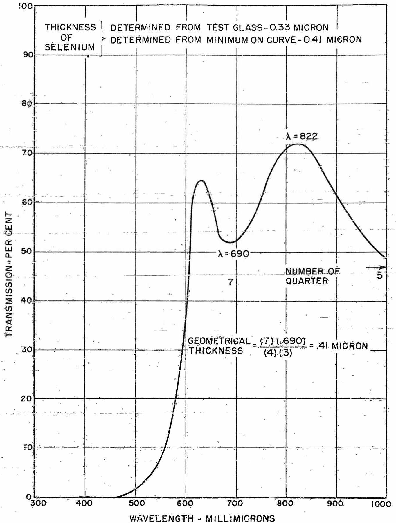
FIGURE 100. TRANSMISSION OF SELENIUM FILM ON GLASS
