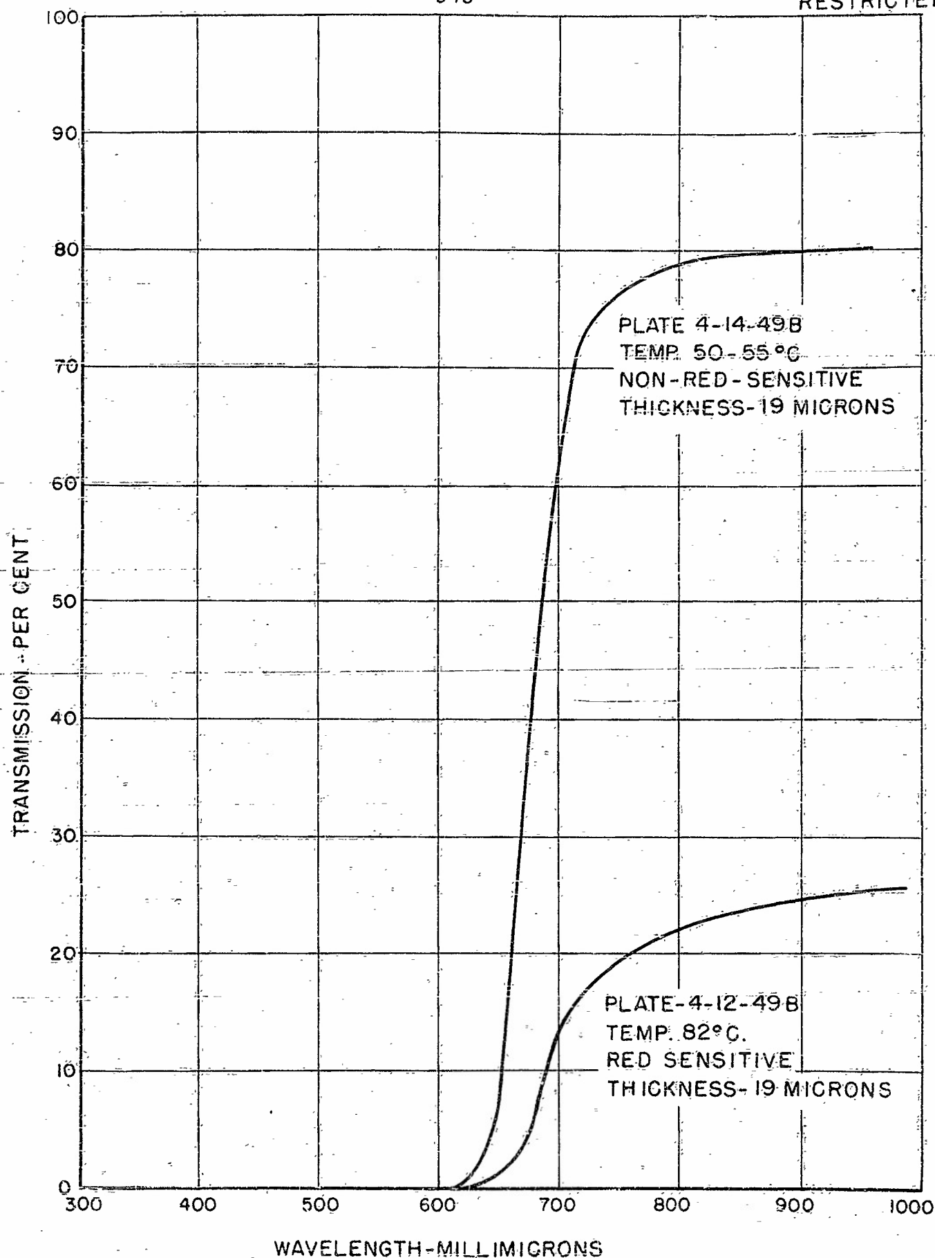
FIGURE 105. TRANSMISSION OF RED-SENSITIVE AND NON-RED-SENSITIVE SELENIUM FILMS-REPRESENTATIVE CURVES
