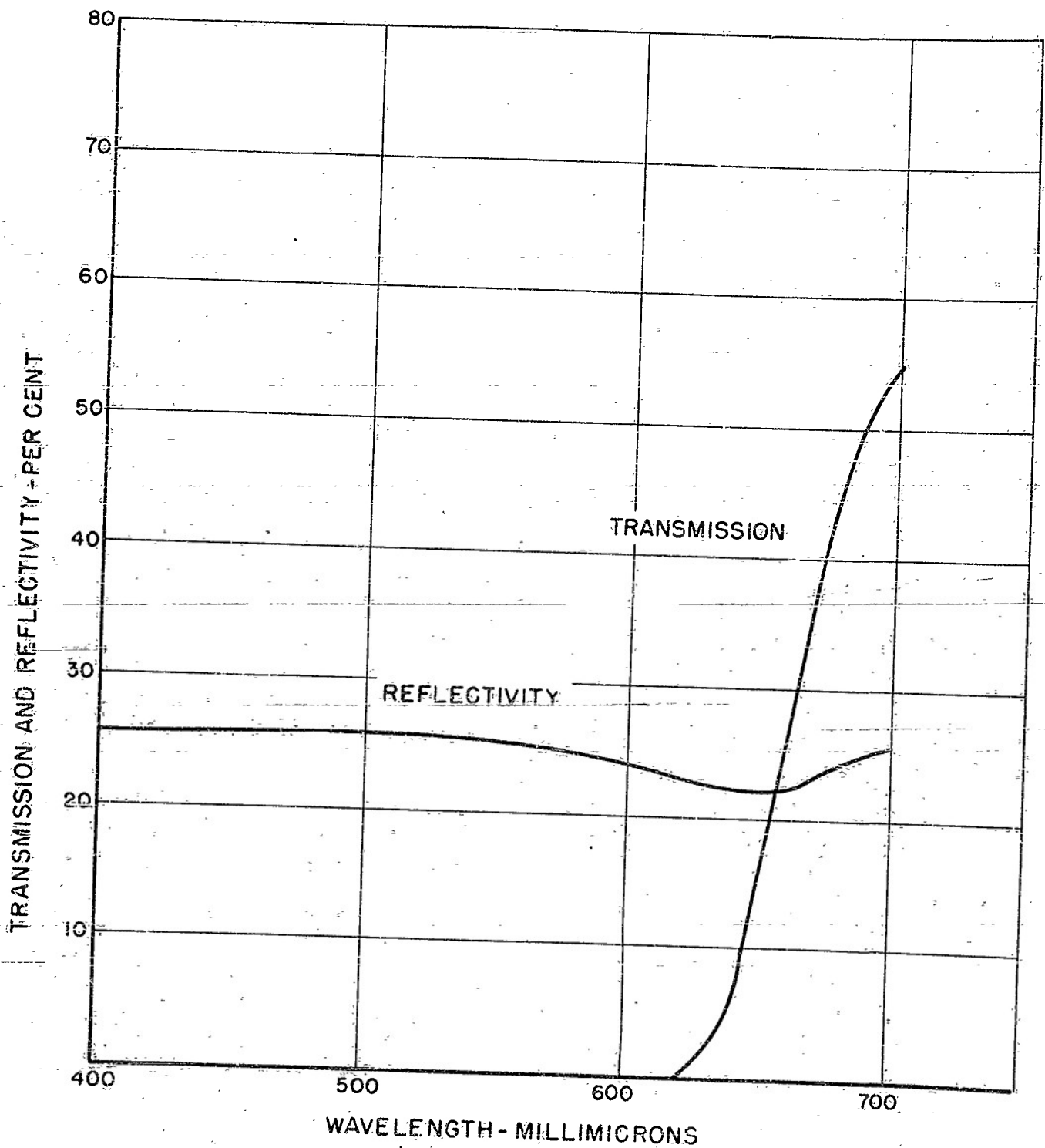
FIGURE 106. TRANSMISSION AND REFLECTIVITY OF SELENIUM FILM ON GLASS
