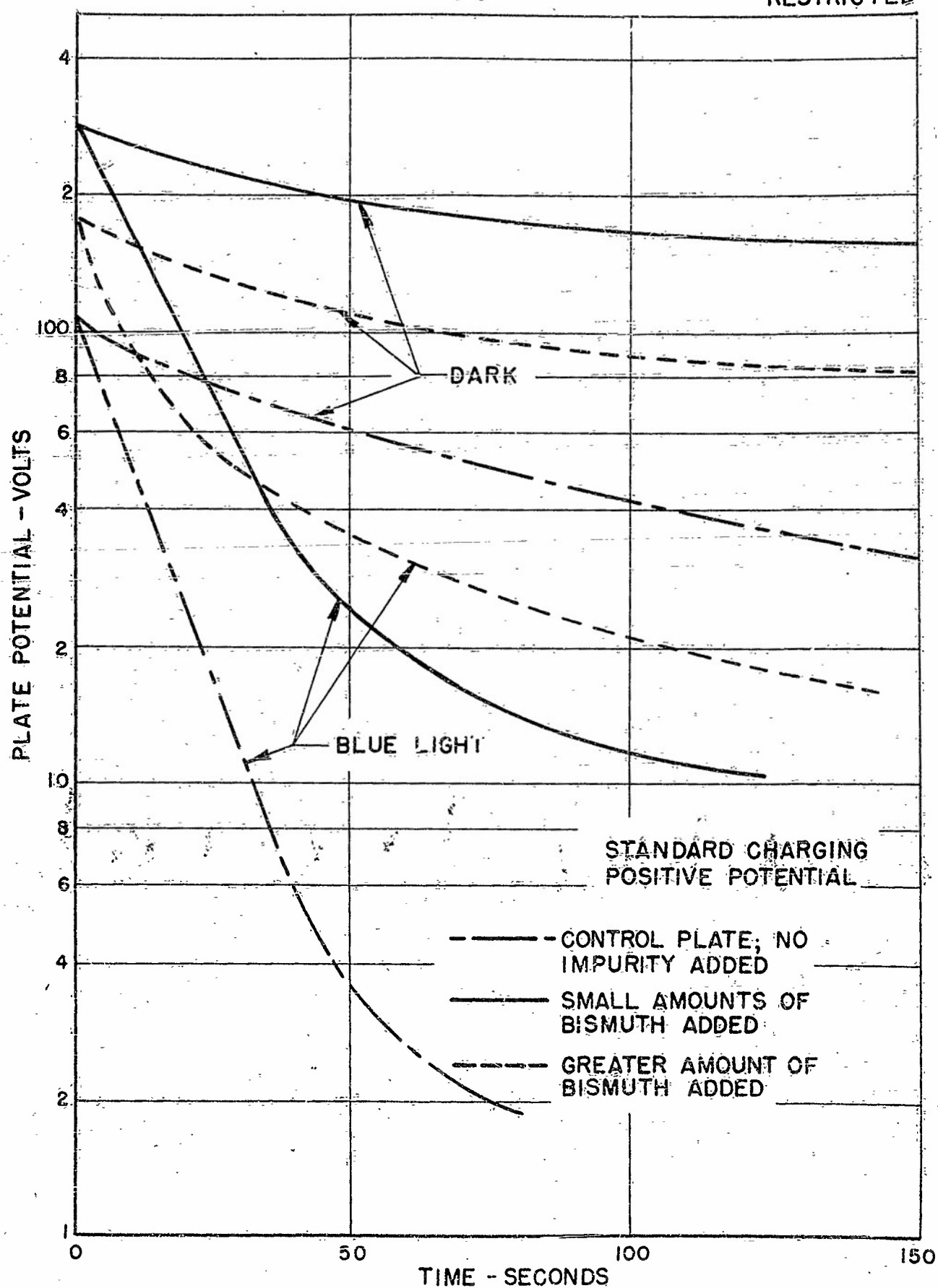
FIGURE 113. BISMUTH-SELENIUM ELECTROPHOTOGRAPHIC PLATES, POSITIVE POTENTIAL DECAY CURVES
