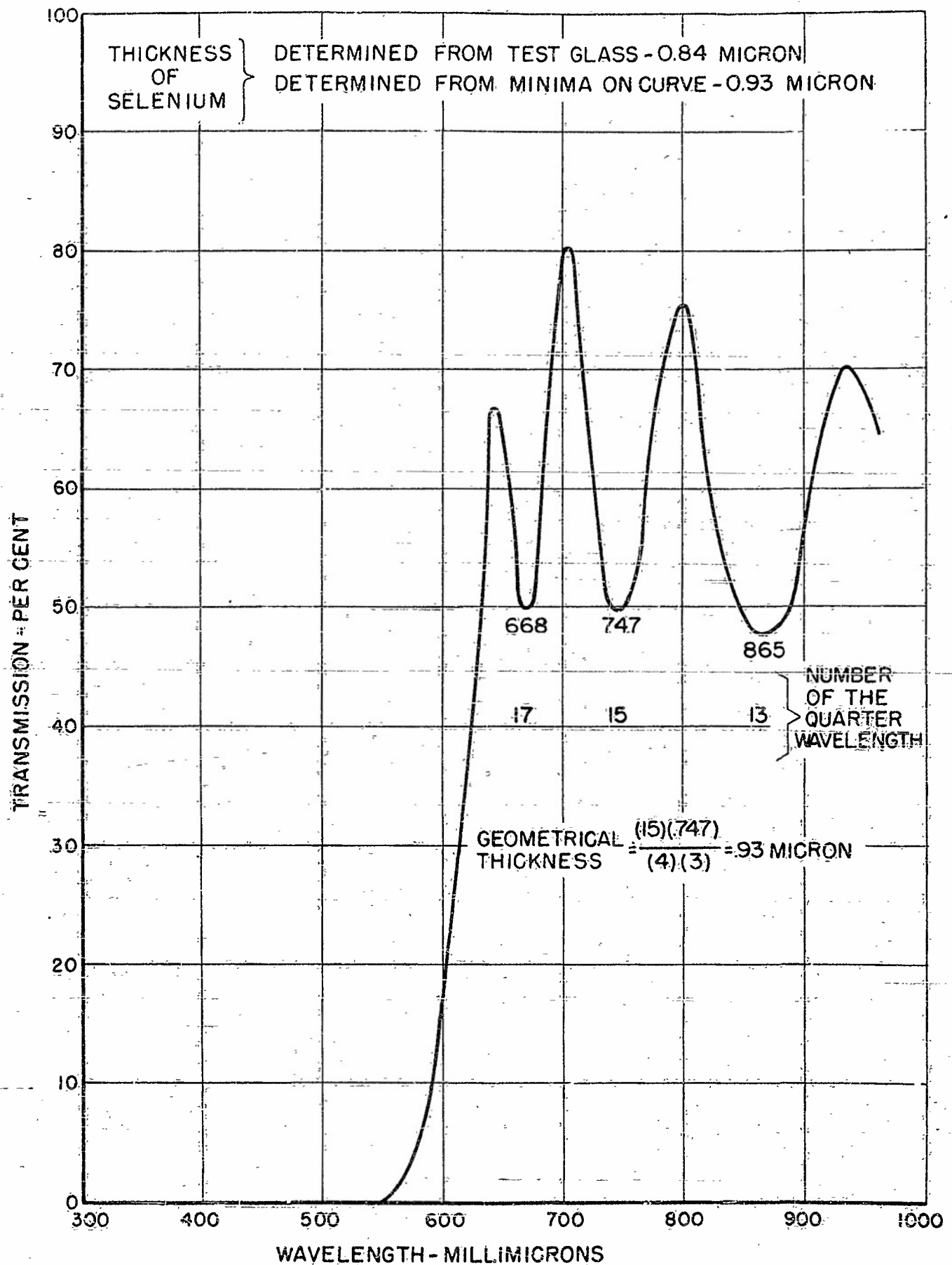
FIGURE 101. TRANSMISSION OF SELENIUM FILM ON GLASS
