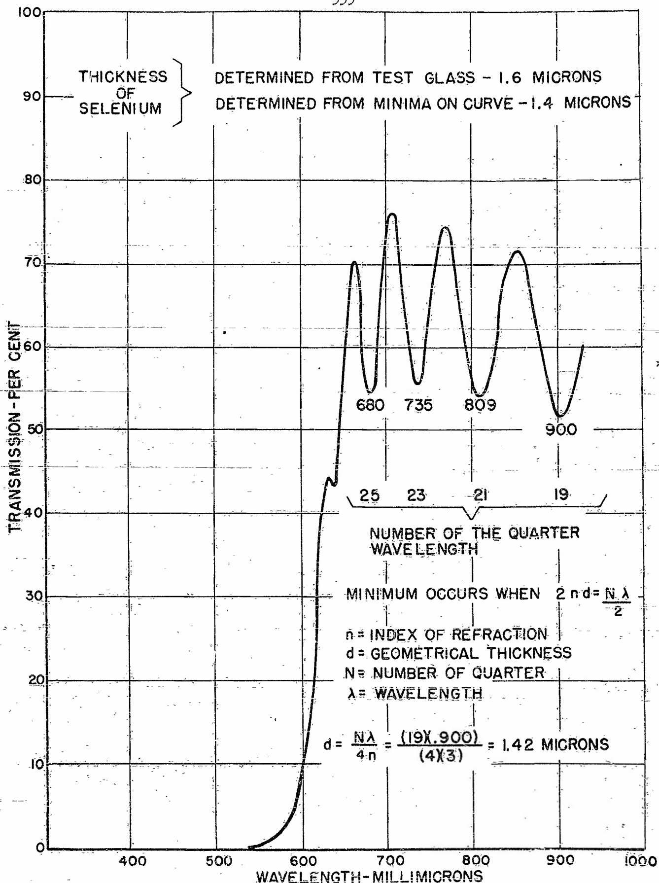
FIGURE 102. TRANSMISSION OF SELENIUM FILM ON GLASS
