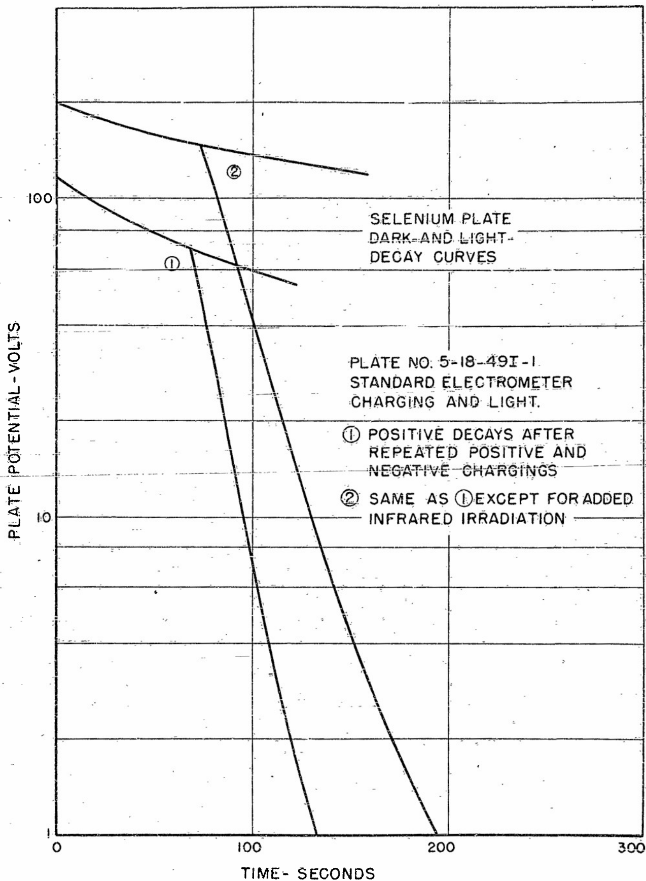
FIGURE 109. EFFECT OF INFRARED IRRADIATION ON A SELENIUM ELECTROPHOTOGRAPHIC PLATE
