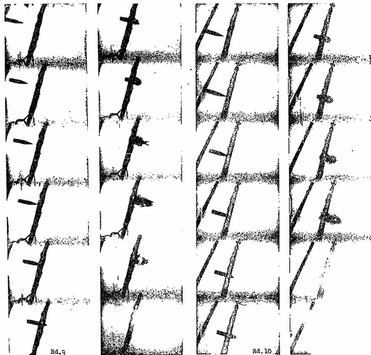
Figure 1. Test of Shell, 105mm, HE, M1. Impacting a 3" wood target. Reproduced from Ultra High-Speed Motion Pictures, (8000 pictures per second).
