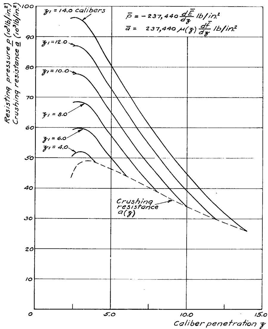
Fig. 10. Resisting pressure p (—) and crushing resistance q (---) versus instantaneous caliber penetration \bar{z} during penetration.
