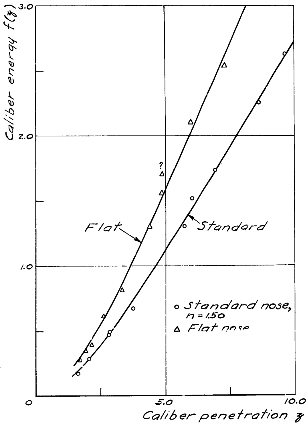
Fig. 4. Penetration data on target cubes B3B3-7.
