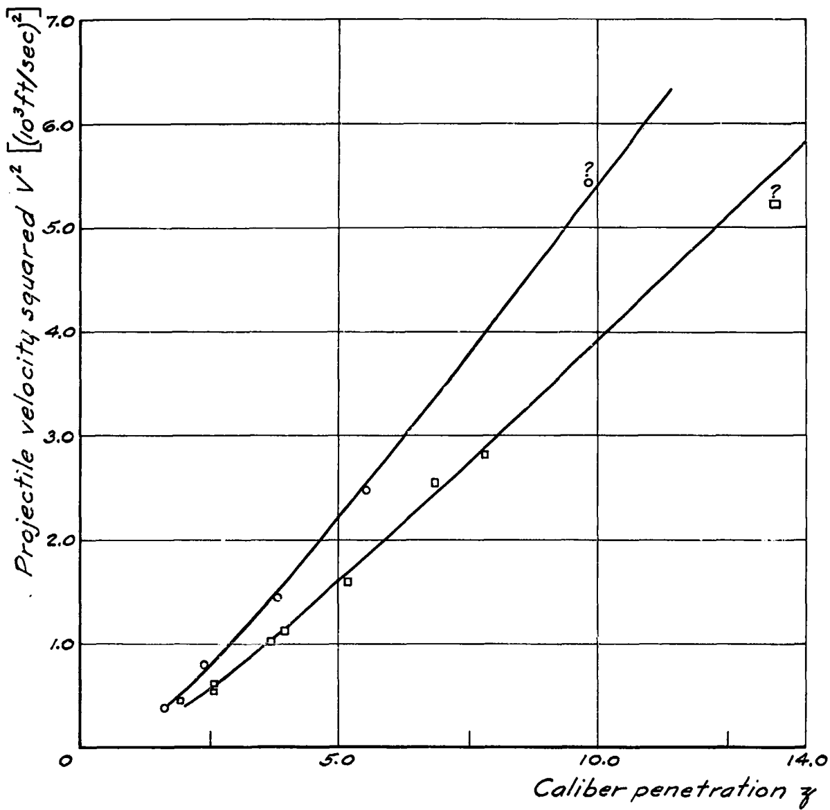
Fig. 7. Penetration data on target cubes B3B 25-29.
