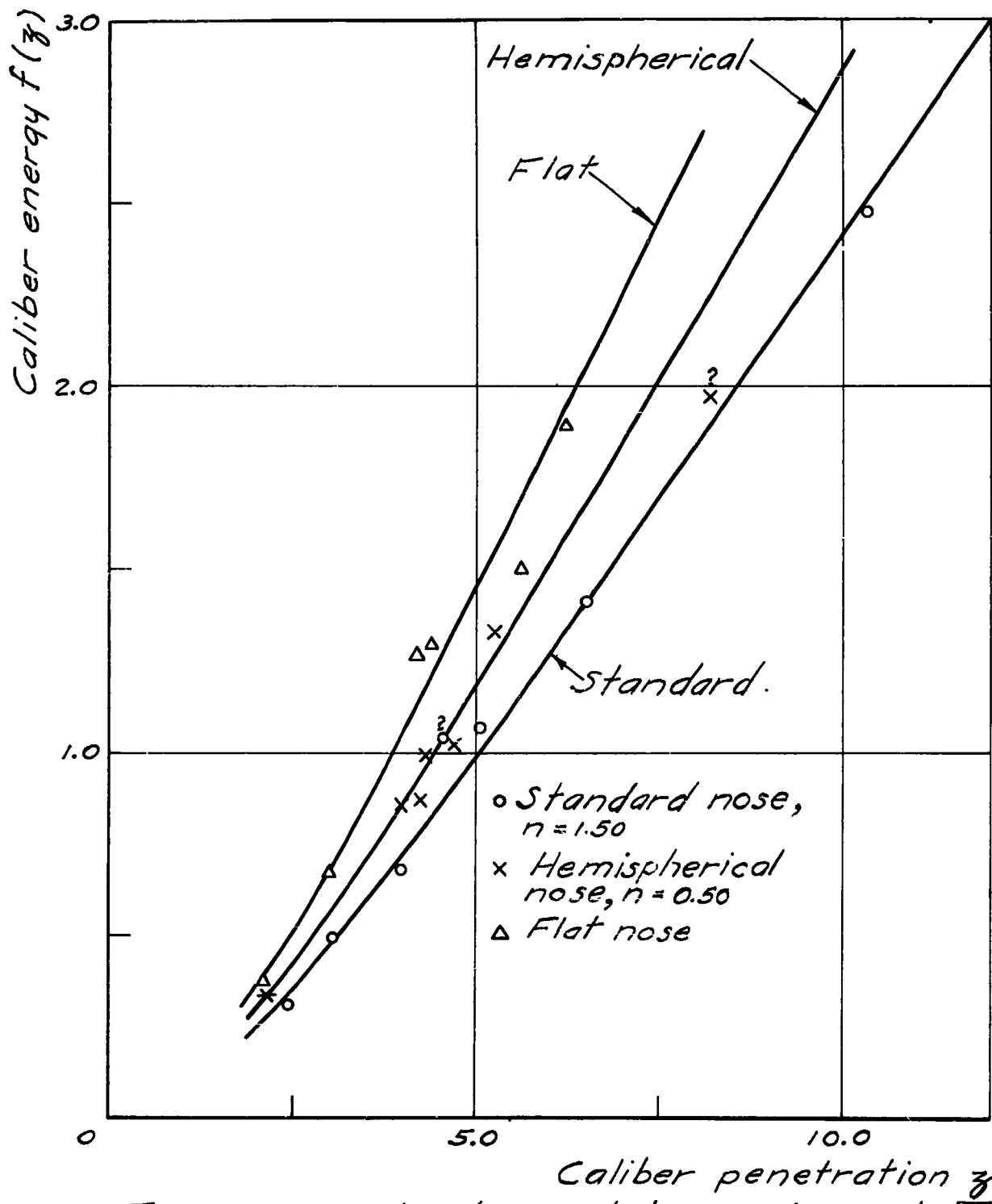
Fig. 5. Penetration data on target cubes B3B13-17.
