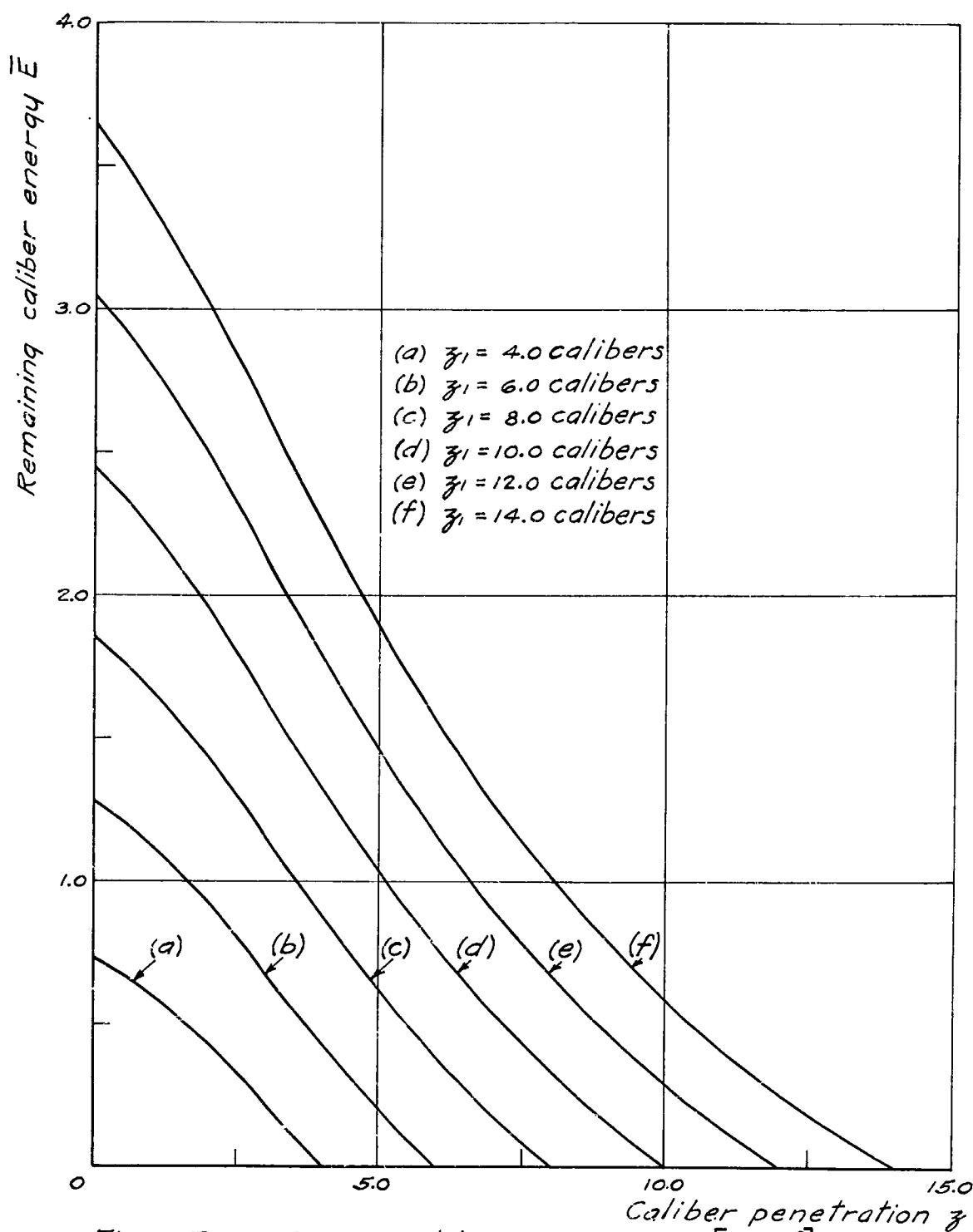
Fig. 9. Remaining caliber energy \bar{E} [= DV^2] versus instantaneous caliber penetration z during penetration. \bar{E} = \mu(z) [\bar{f}(z_1) - \bar{f}(z)] . The curves are based on the average caliber .50 E-6 penetration curve \bar{f}(z) = \bar{f}(z) given in Table I and Fig. 2, and on \gamma = 0.6 .
