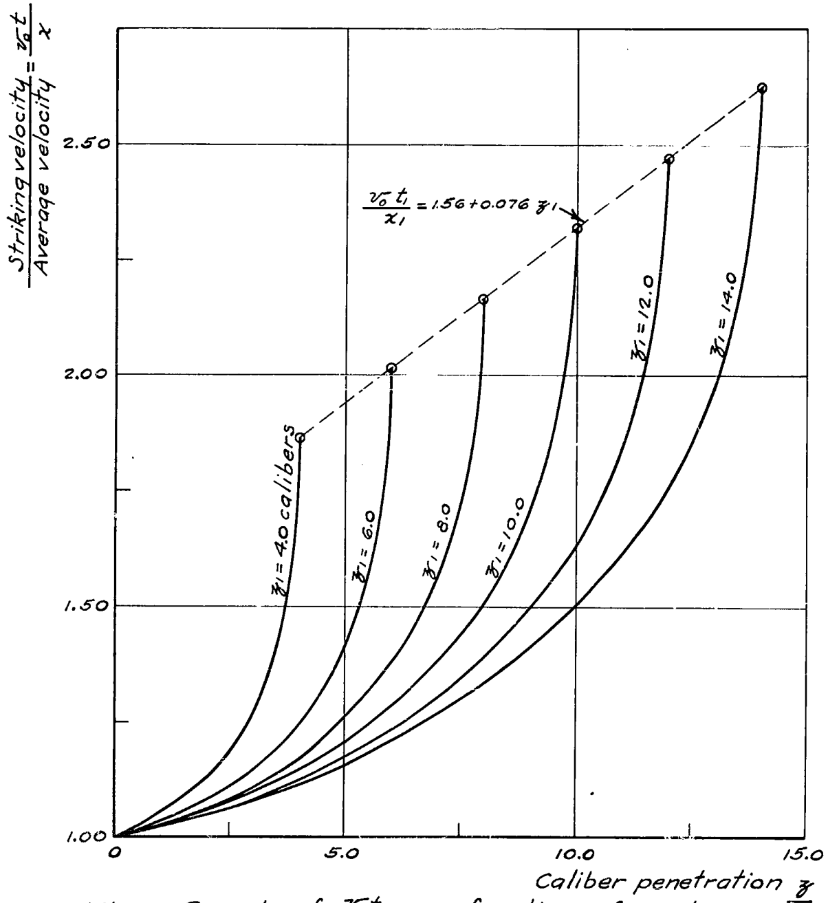
Fig. 11. Graph of \frac{v_0 t}{x} as a function of z_1 during penetration.
