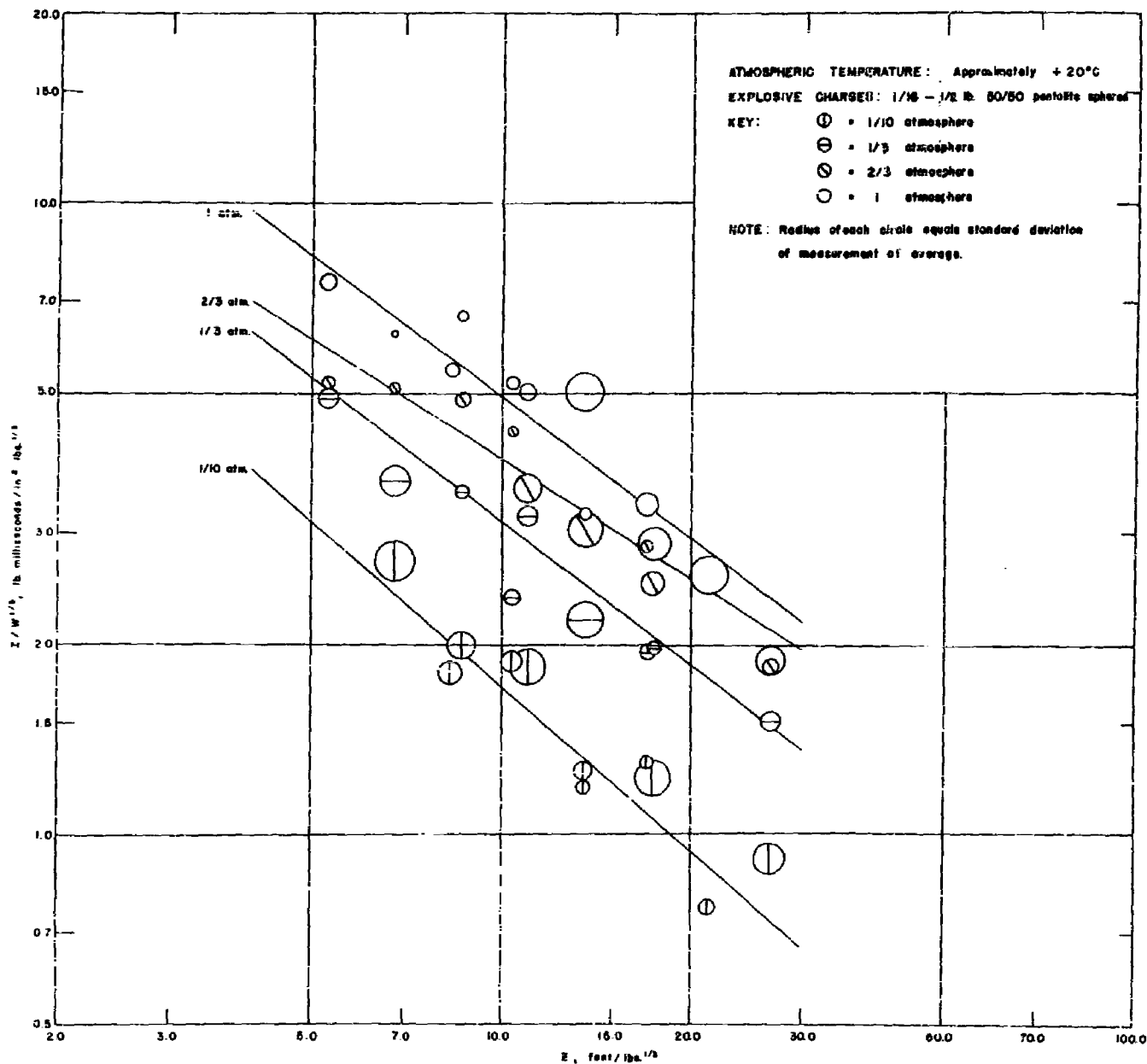
FIGURE 8 IMPULSE / (CHARGE WEIGHT) 1/3 vs. Z = DISTANCE / (CHARGE WEIGHT) 1/3 at DIFFERENT ATMOSPHERIC PRESSURES
