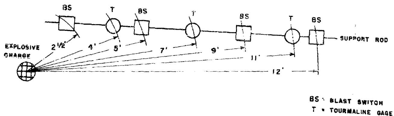
Figure 1. Schematic Diagram of Gage Set - Up (Dimensions are approximate)
