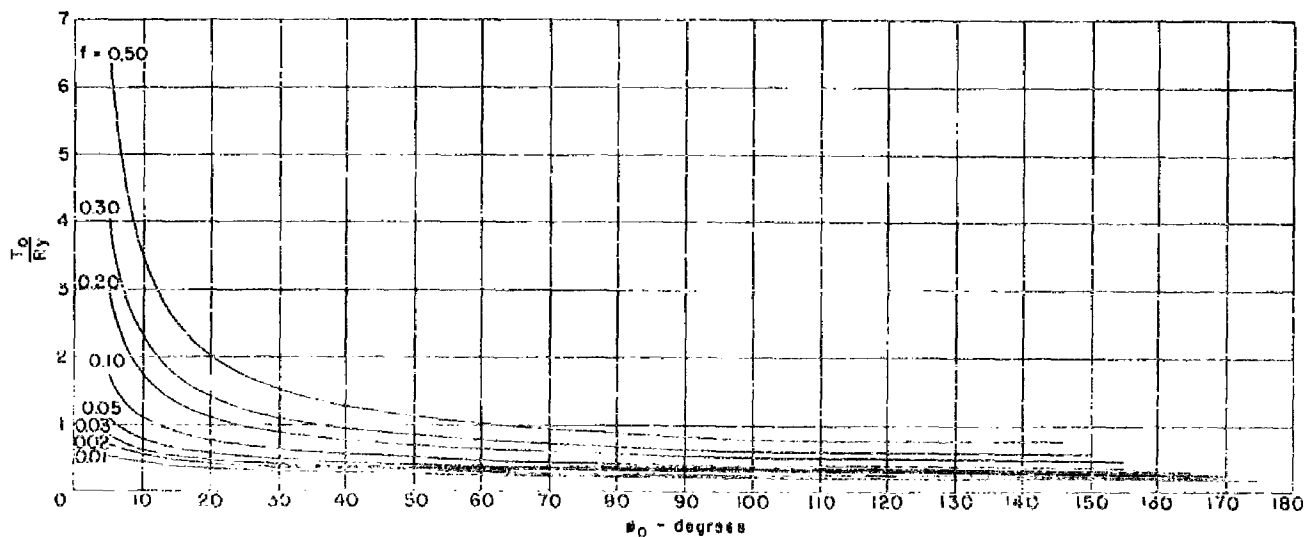
Figure 3c - Variation of T_0/Ry with \phi_0 and f .
