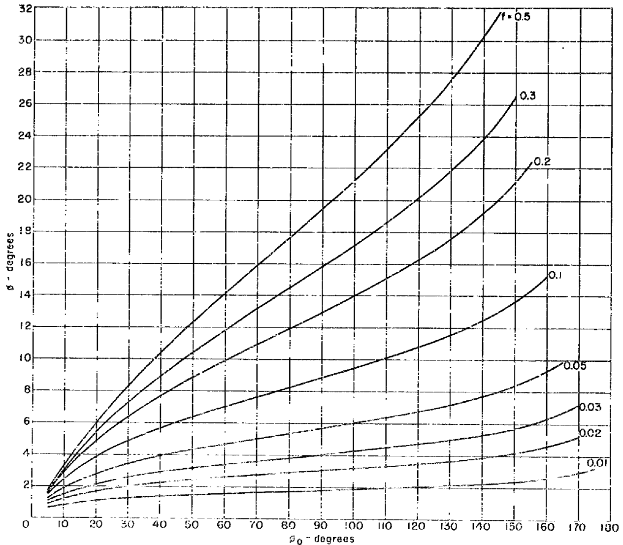
Figure 3a - Variation of \phi with \phi_0 and r .
