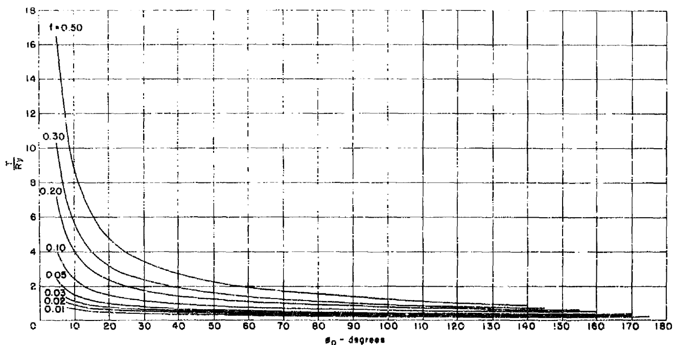
Figure 3b - Variation of T/Ry with \phi_0 and f .
