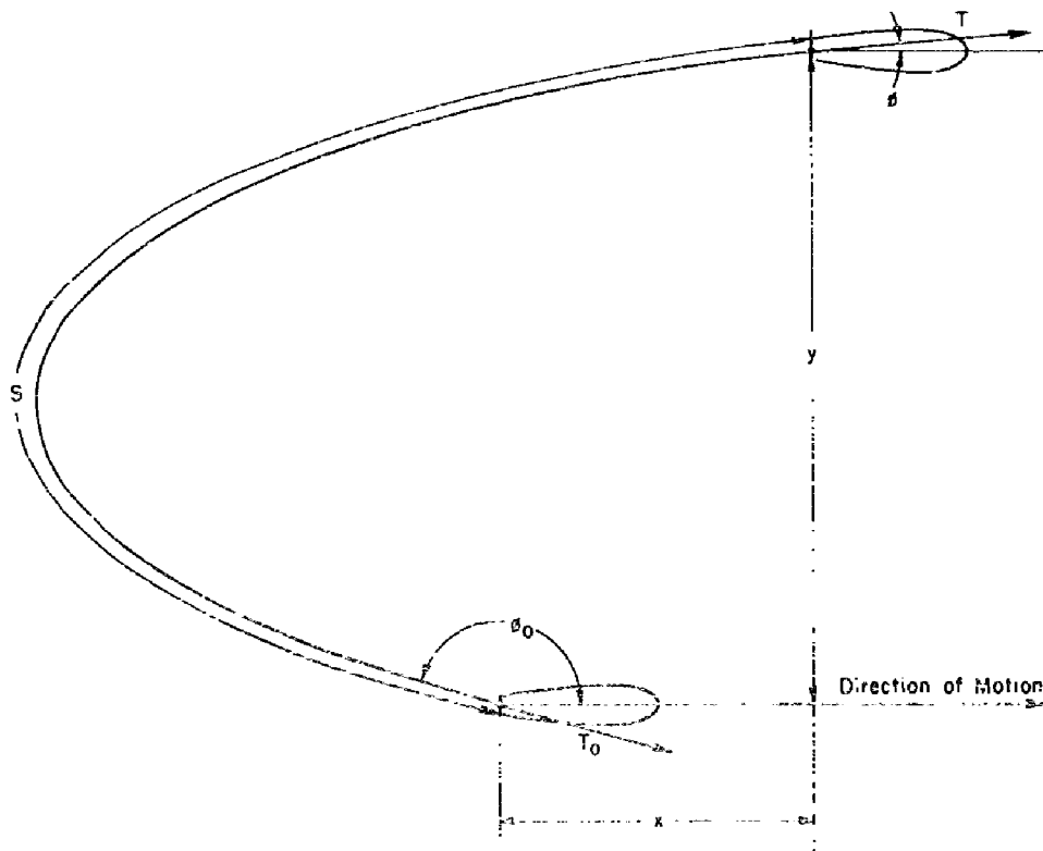
Figure 2 - Cable Configuration for Two Powered Vessels
