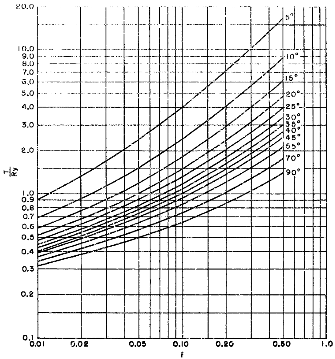
Figure 3f - Variation of T/Ry with \theta_0 and f .
