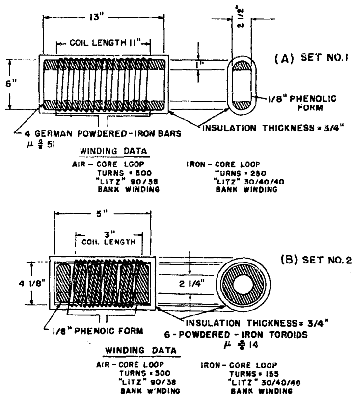
Figure 5 - Schematic structural diagram of experimental iron-core loop antennas
