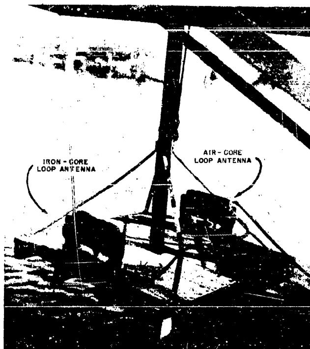
Figure 6 - The set No. 1 rubber-covered loop antennas
