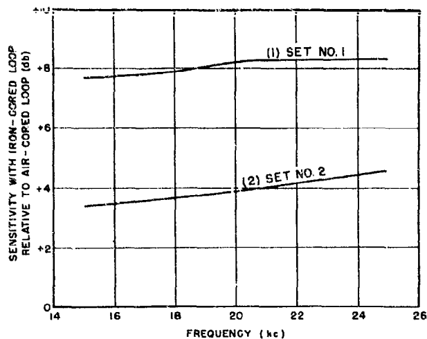
Figure 13 - Laboratory tests-initial over-all receiver-sensitivity comparisons for loop-antenna sets Nos. 1 and 2, wax-covered, in air
