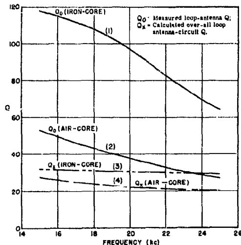
Figure 11 - Laboratory tests-initial Q values of the wax-covered set No. 1 loop antennas in air
