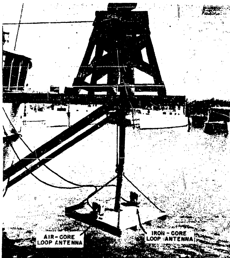
Figure 4 - The set No. 2 wax-covered loop antennas
