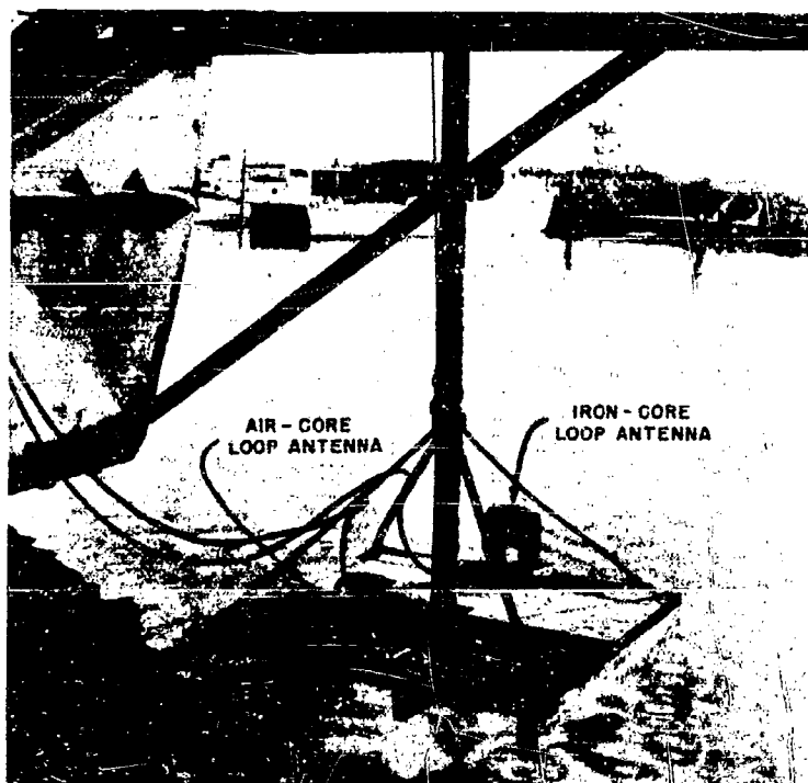
Figure 7 - The set No. 2 rubber-covered loop antennas
