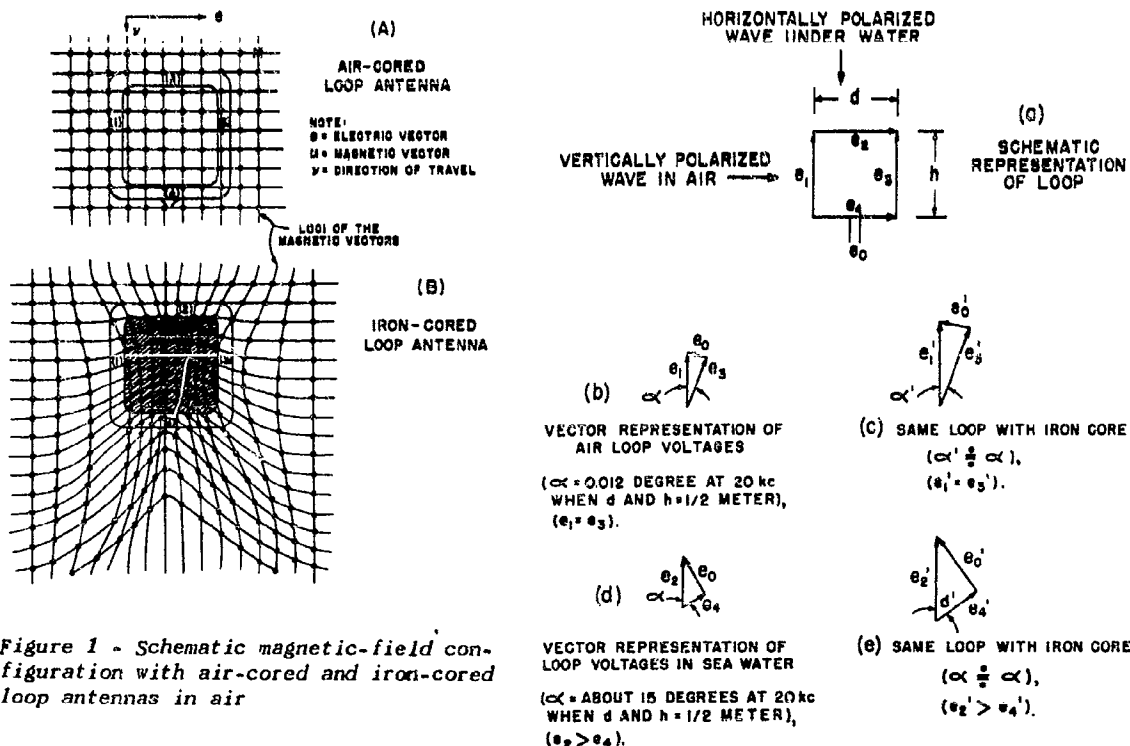
Figure 2 - Loop induced voltages
