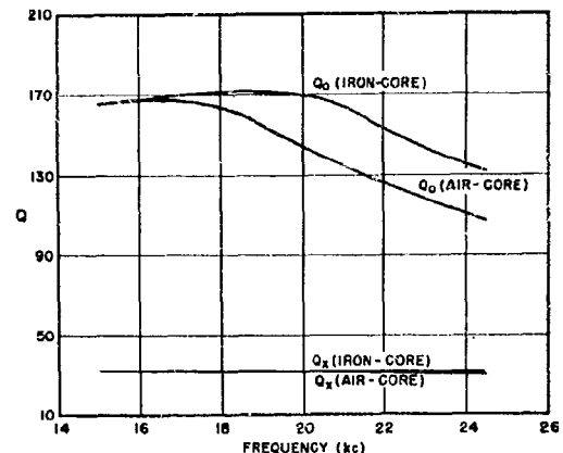
Figure 12 - Laboratory tests-initial Q values of wax-set No. 2 loop antennas in air
