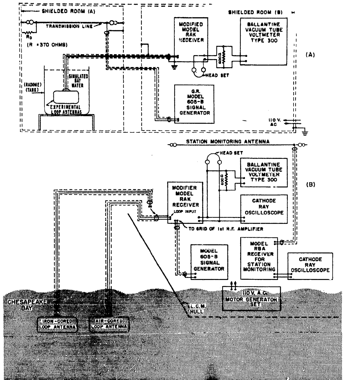
Figure 8 - Equipment arrangement for laboratory and Chesapeake Bay measurements of submerged loop performance
