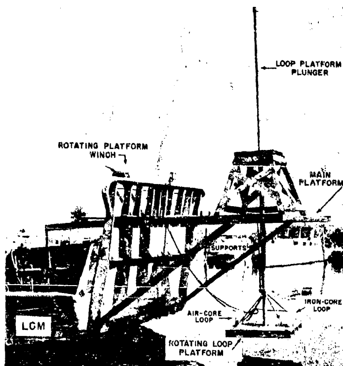
Figure 10 - LCM landing-craft platform and rigging construction
