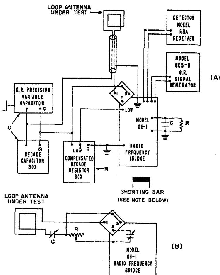
(A) Block Diagram of Equipment for Measurement of Loop Antenna R-F Resistance and Resonating Capacitance.
