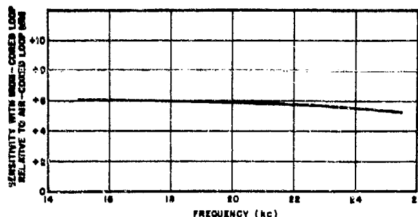
Figure 14 - Laboratory tests-over-all receiver-sensitivity comparison for rubber-covered, set No. 1 loop antennas
