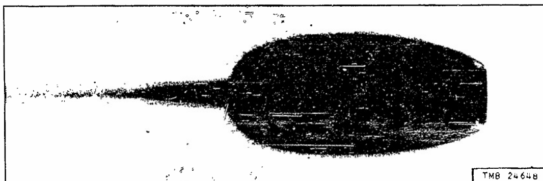
Figure 1 - Time Exposure of the Cavitation Bubble Formed Behind a Disc at \sigma_0 = 0.255
