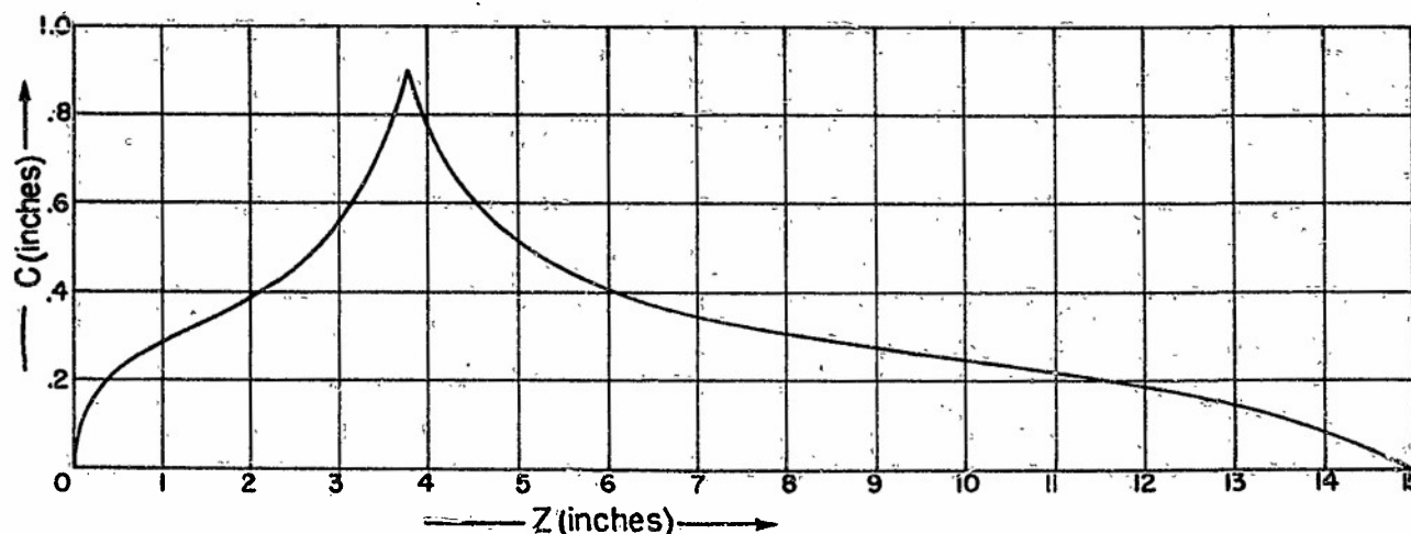
Fig. 8. Thickness of polystyrene loading vs z .
