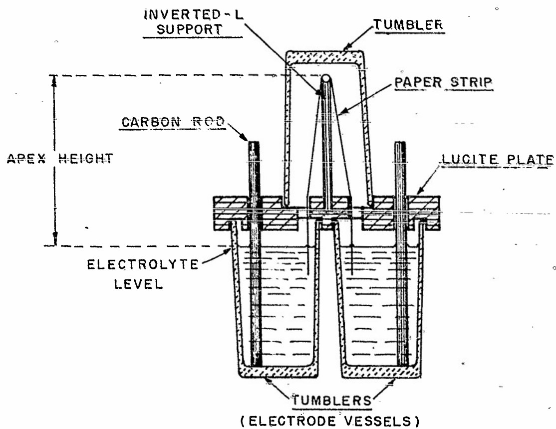
FIG. 1. DIAGRAM OF APPARATUS.
