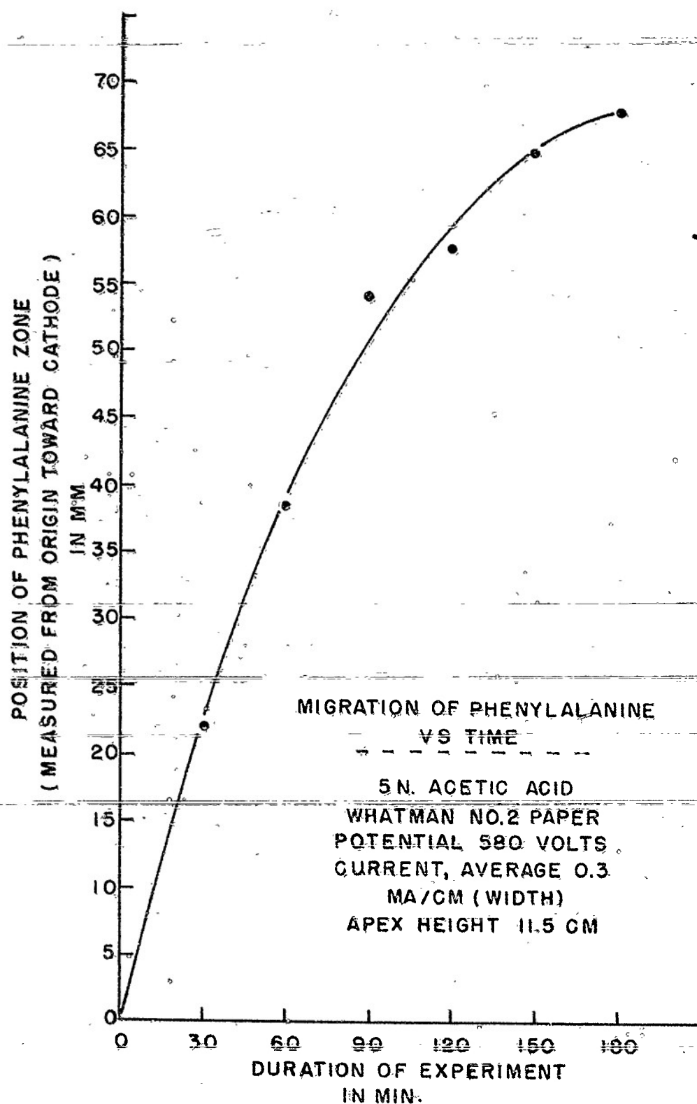
FIG.7 MIGRATION OF PHENYLALANINE (EXP. VII)
