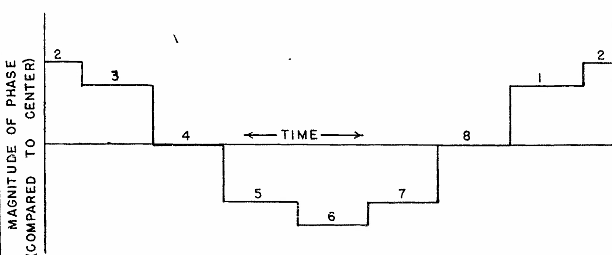
PHASE RELATIONS OF COMMUTATED ANTENNAS
