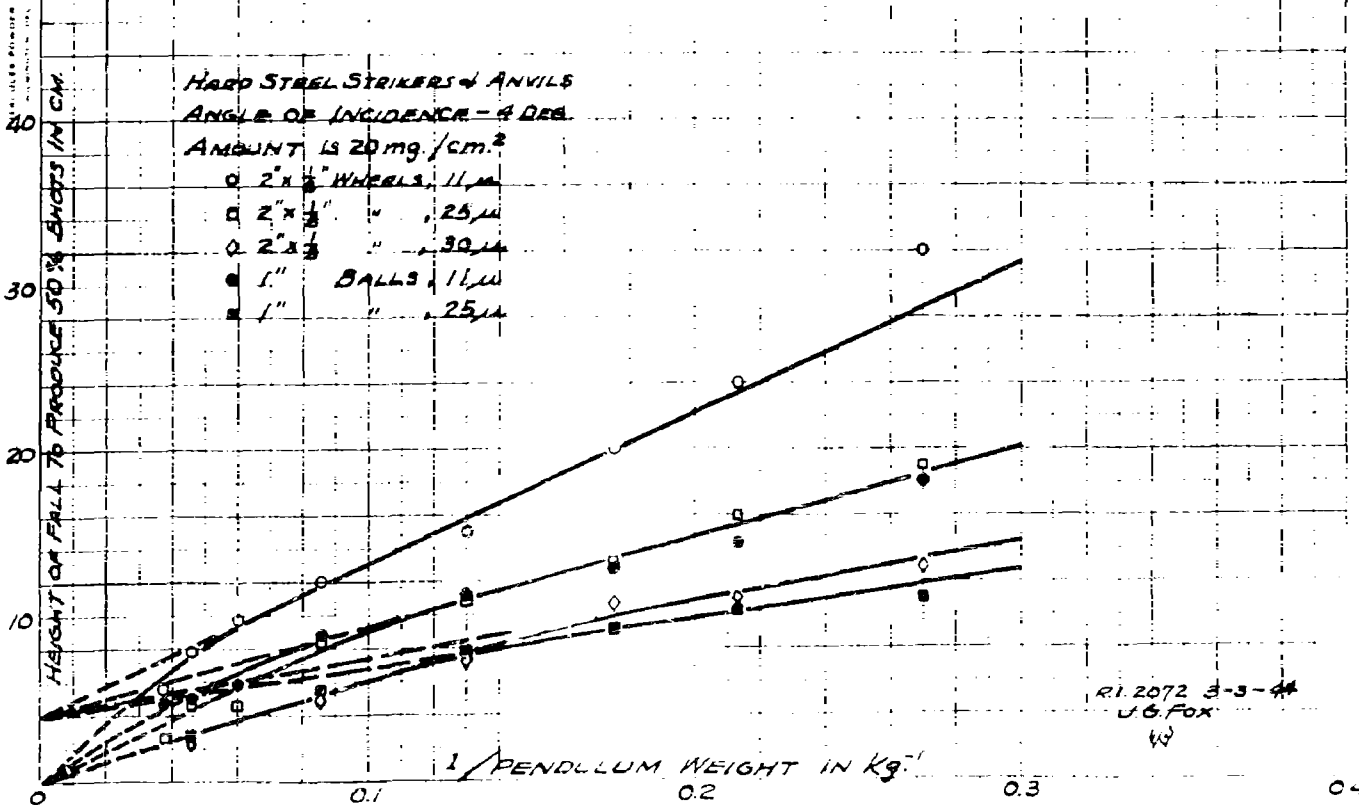
FIGURE 2 VARIATION OF HEIGHT OF FALL WITH PENDULUM WEIGHT FOR CYCLONITE THROUGH 325
