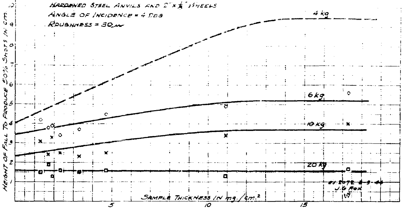
FIGURE 2 VARIATION OF HEIGHT OF FALL WITH PENDULUM WEIGHT FOR CYCLONITE THROUGH 325
