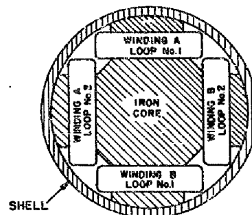
(b) FOUR-WINDING SPACED TYPE (TOP VIEW) (WINDINGS A AND B IN SERIES FOR EACH LOOP)
