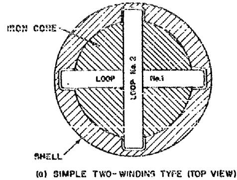
(a) SIMPLE TWO-WINDING TYPE (TOP VIEW)
