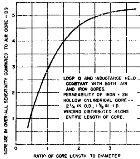
Figure 14 - Measured effect of iron-dust core on loop efficiency
