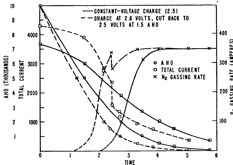
Figure 14 - Constructed charge data for charge at 90^{\circ} F, OWTX cell
