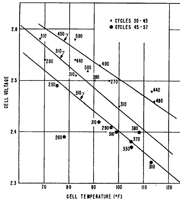
Figure 6 - Full-charge gassing data; numbers at points are H 2 gassing rates in amperes
