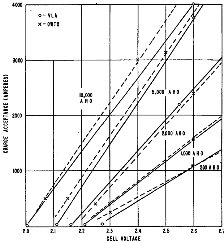
Figure 11 - Charge acceptance vs. cell voltage, VLA and OWTX cells
