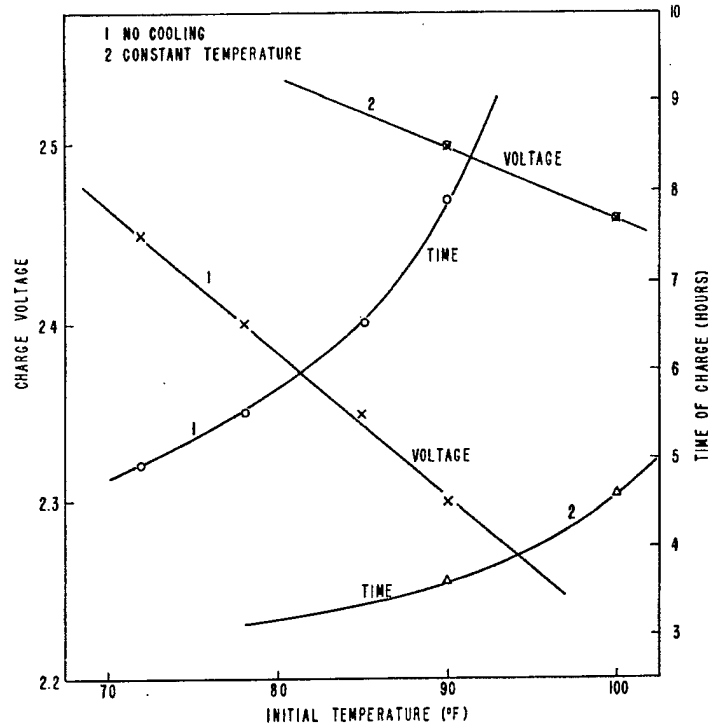
Figure 26 - Comparison of charge times and voltages for efficient cooling and no cooling, 7,000 AHO, MAQ cell
