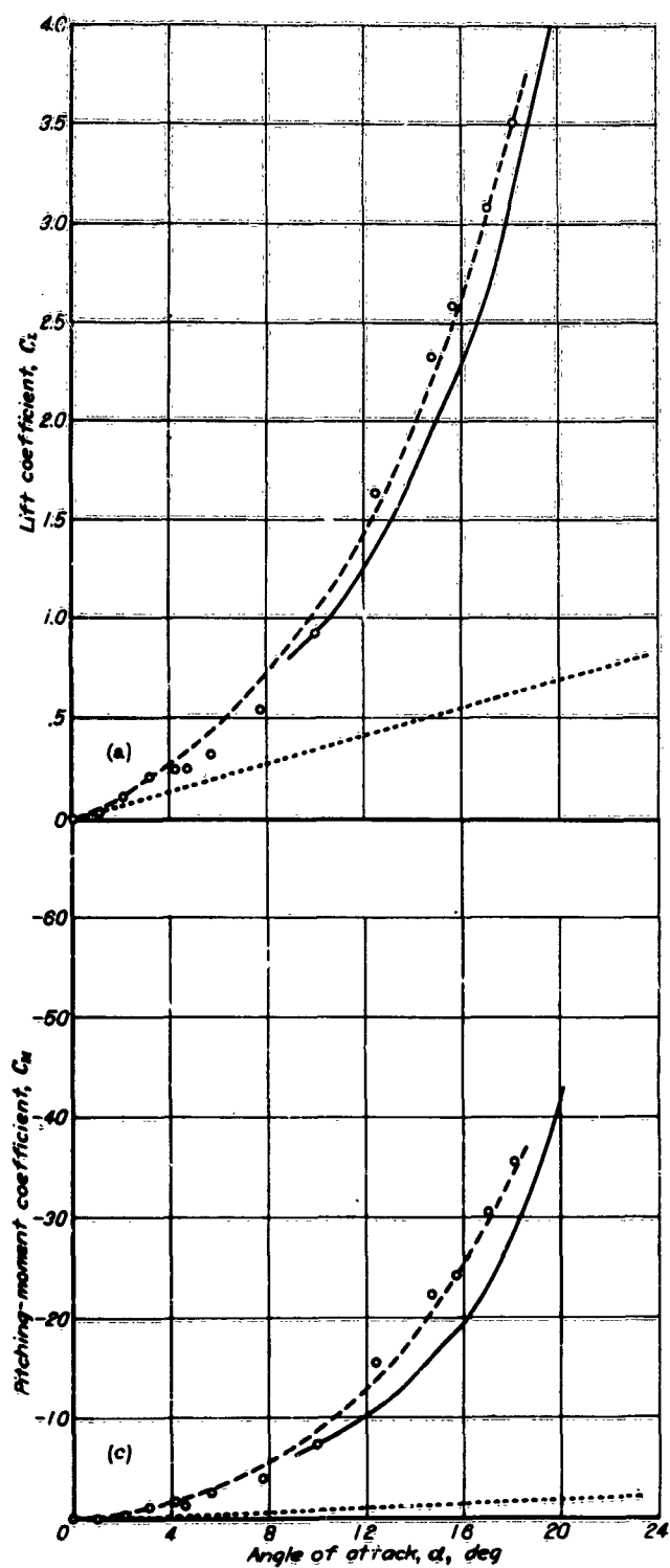
FIGURE 7.—Force, moment, and center-of-pressure characteristics for body I (fineness ratio 21.1).
