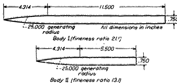
FIGURE 6.—Bodies of revolution.
