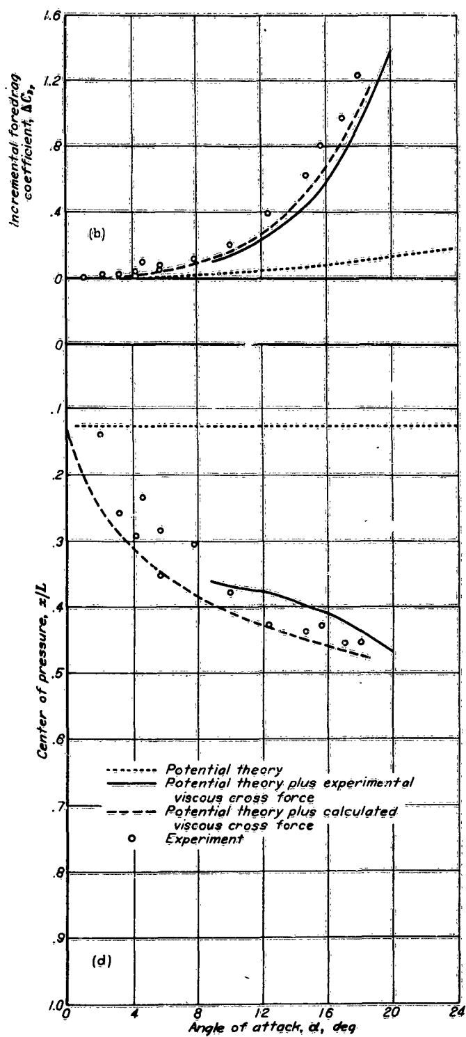
FIGURE 7.—Force, moment, and center-of-pressure characteristics for body I (fineness ratio 21.1).
