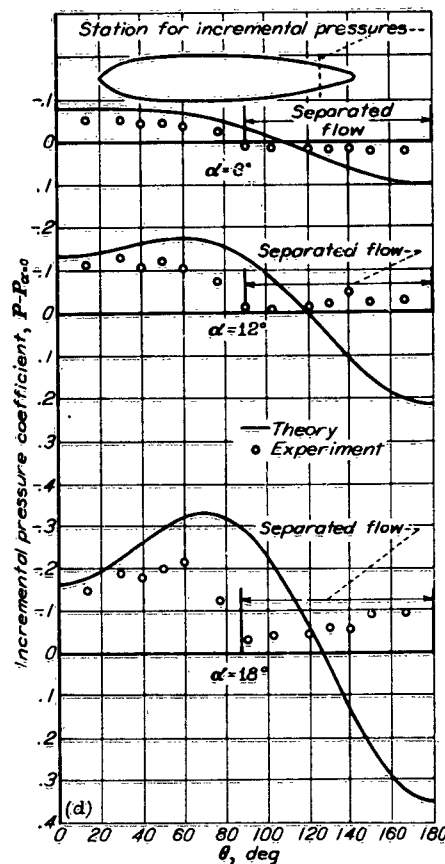
FIGURE 2—Calculated and experimental pressure distribution on a model hull of the U. S. S. Akron.
