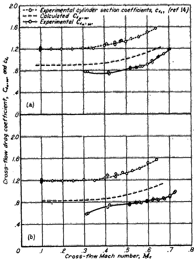
FIGURE 9.—Comparison of calculated cross-flow drag coefficients at 90° angle of attack with experimental values obtained from Ames 1- by 3½-foot wind tunnel for (a) body I and (b) body II.
