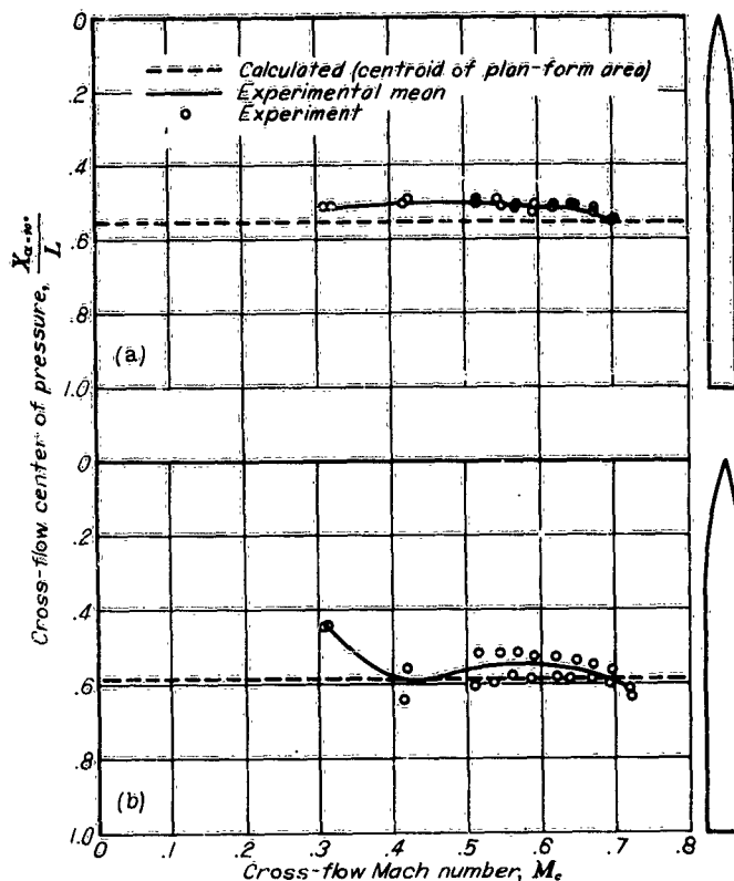
FIGURE 10.—Comparison of calculated centers of pressure at 90° angle of attack with experimental values obtained from Ames 1- by 3½-foot wind tunnel for (a) body I and (b) body II.
