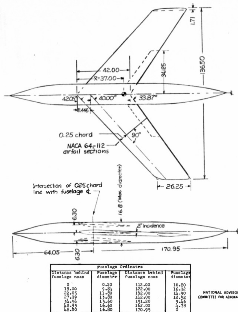
Figure 1.- Geometry of 40° sweptback wing and fuselage.
