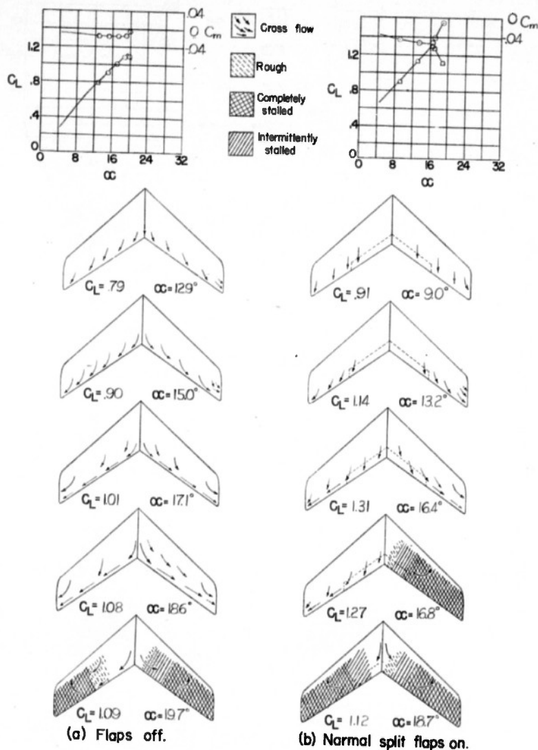
Figure 11.- Stalling characteristics of 40° sweptback wing. R = 6,840,000 .
