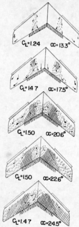
(c) 0.575 b/2 span leading-edge flaps and extended split flaps on.
