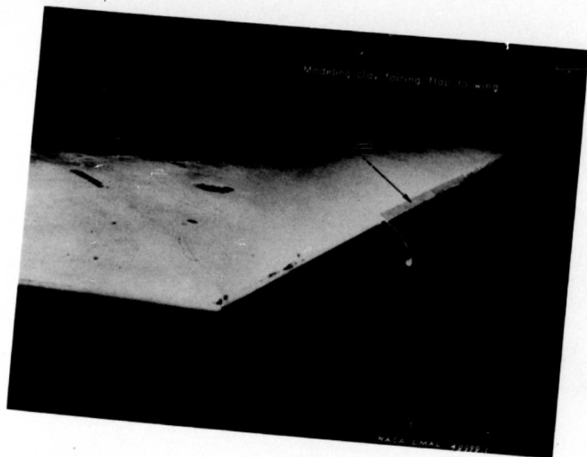
Figure 3.- Leading-edge flap mounted on 40^\circ sweptback wing.
