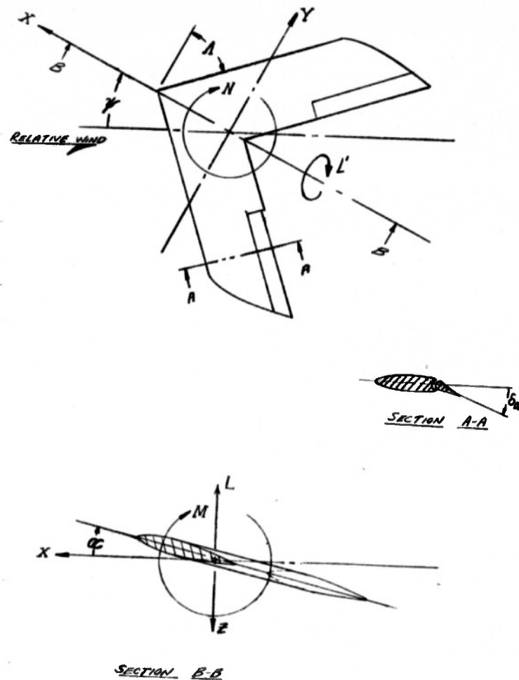
Figure 1.-System of axes used. Positive values of forces, moments, and angles are indicated.
