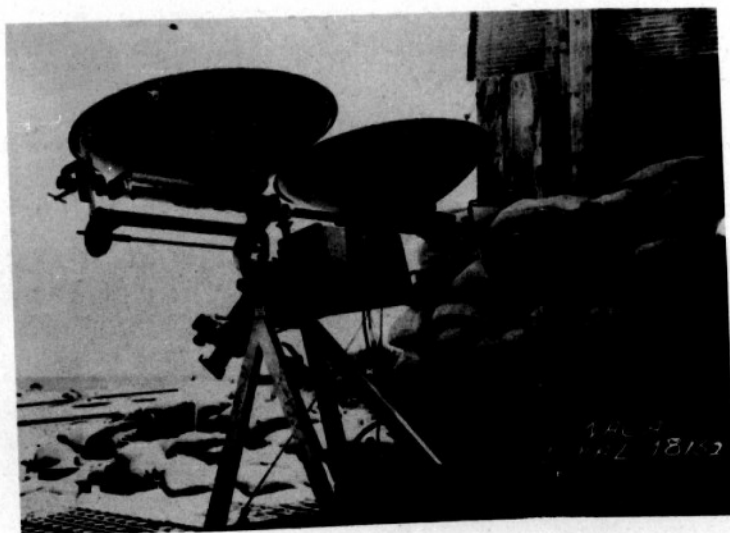
Figure 9.- Continuous-wave Doppler radar set (AN/TPS-5).
