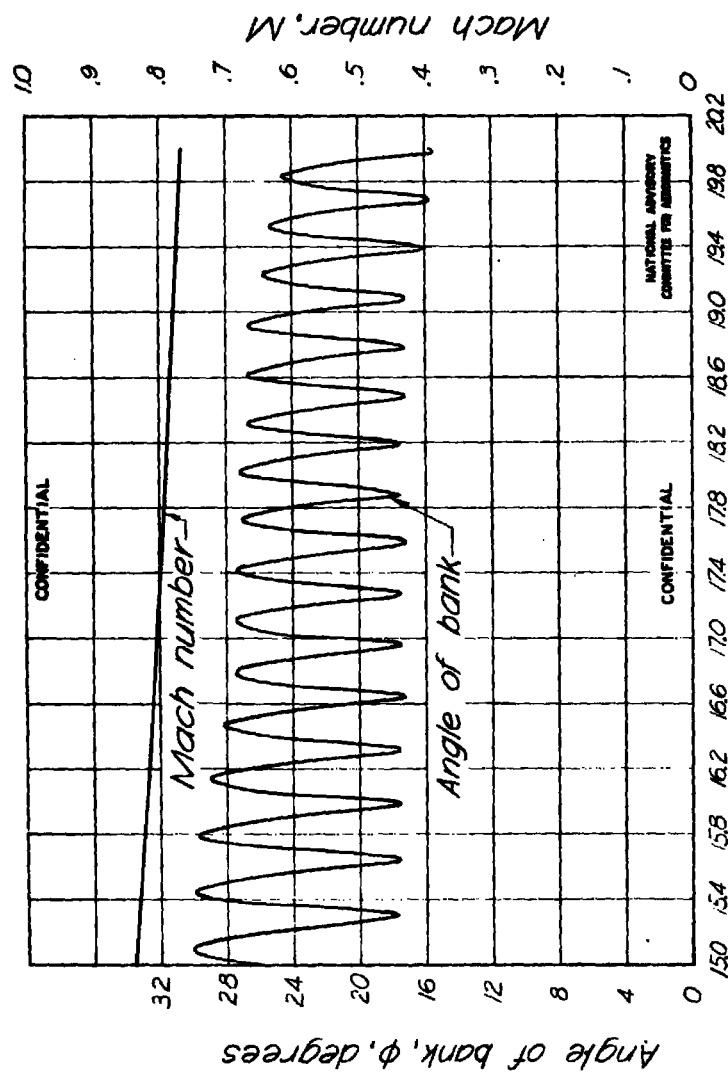
Figure 30.-Telemeter time history of roll characteristics of the RM-1 in flight. Time after launching, t , seconds
