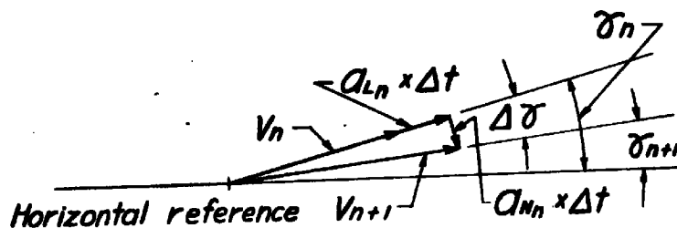
(b) Vectorial representation of iterant flight-path relationships (equation (8)).
