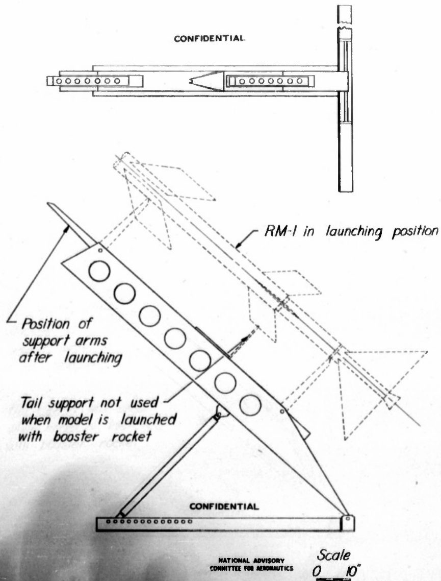
Figure 7. -- RM-1 launching rack.
