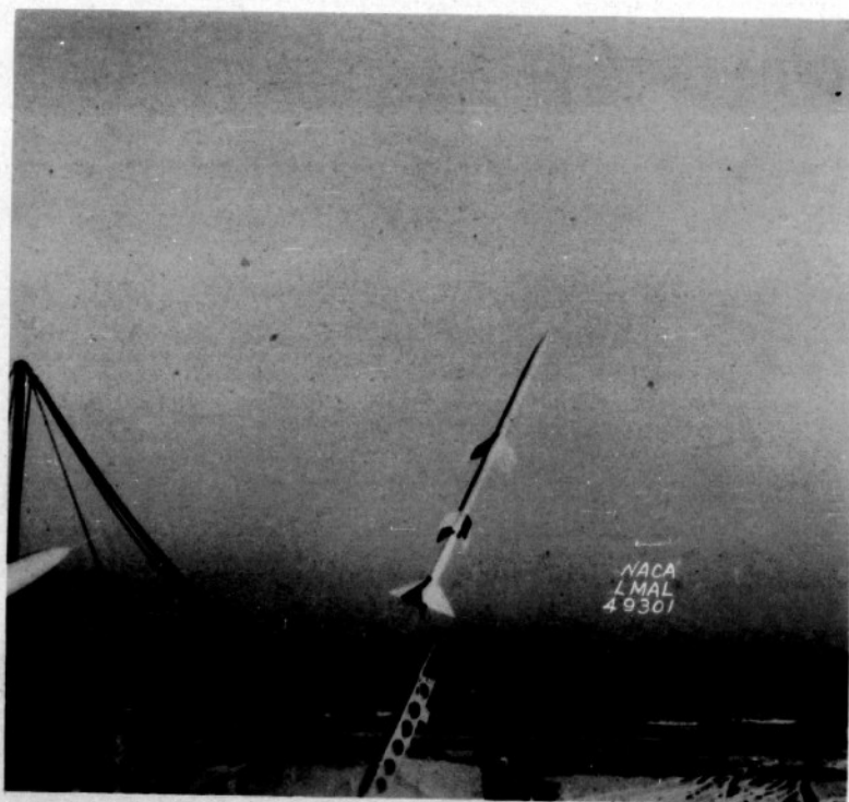
Figure 17.- Launching of RM-1 dummy with booster tail. (First flight)
