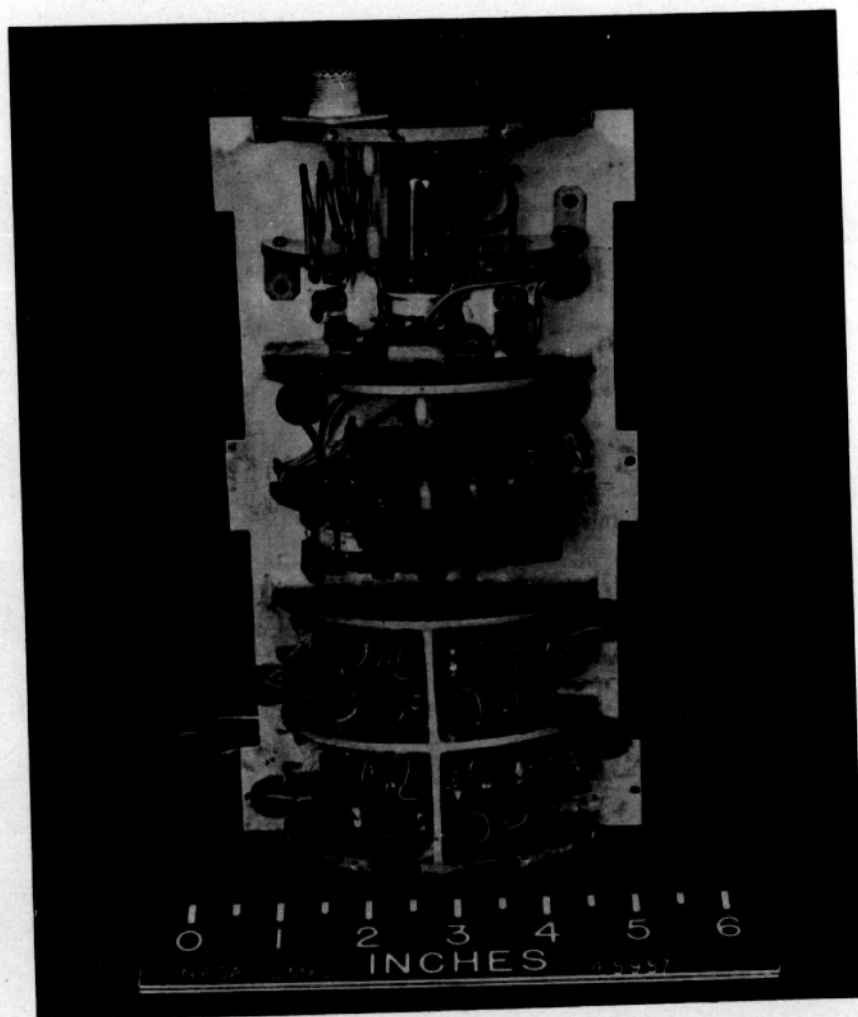
Figure 10.- Radio-transmitter part of RM-1 model four-channel telemeter.
