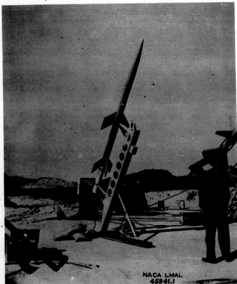
Figure 8.- The RM-1 model with booster tail mounted on launching rack.
