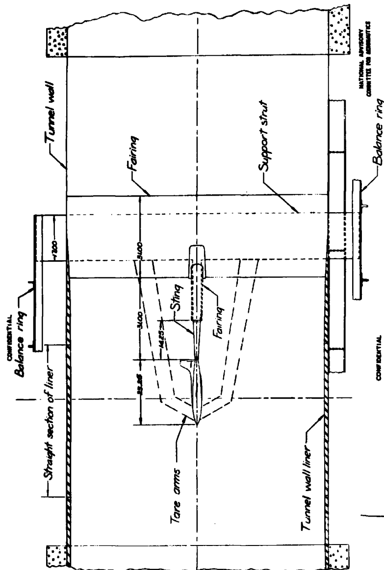
Figure 3.- XS-1 model on sting support in the Langley 8-foot high-speed tunnel.
