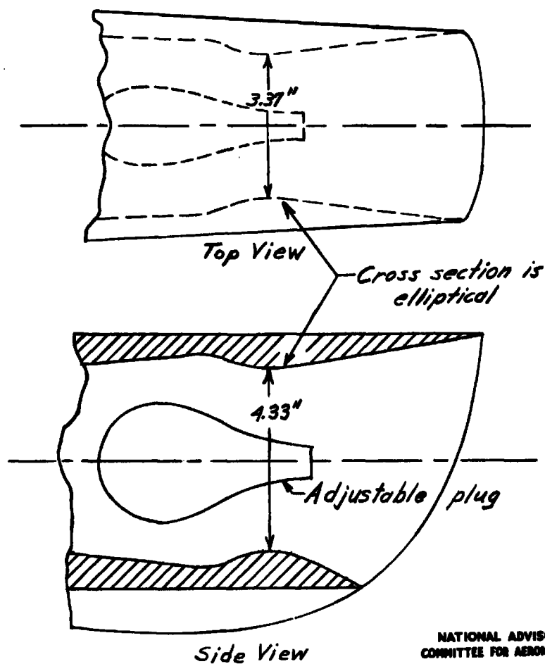
Figure 7.- Original nozzle on complete wind-tunnel model.
